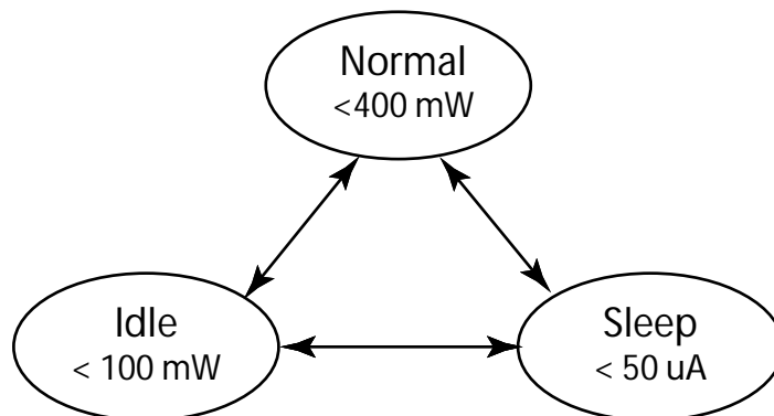
Figure 2: Intel StrongARM SA-1110 Power Consumption
