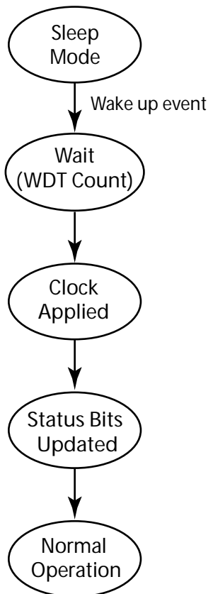
Figure 3: Wake up Sequence
