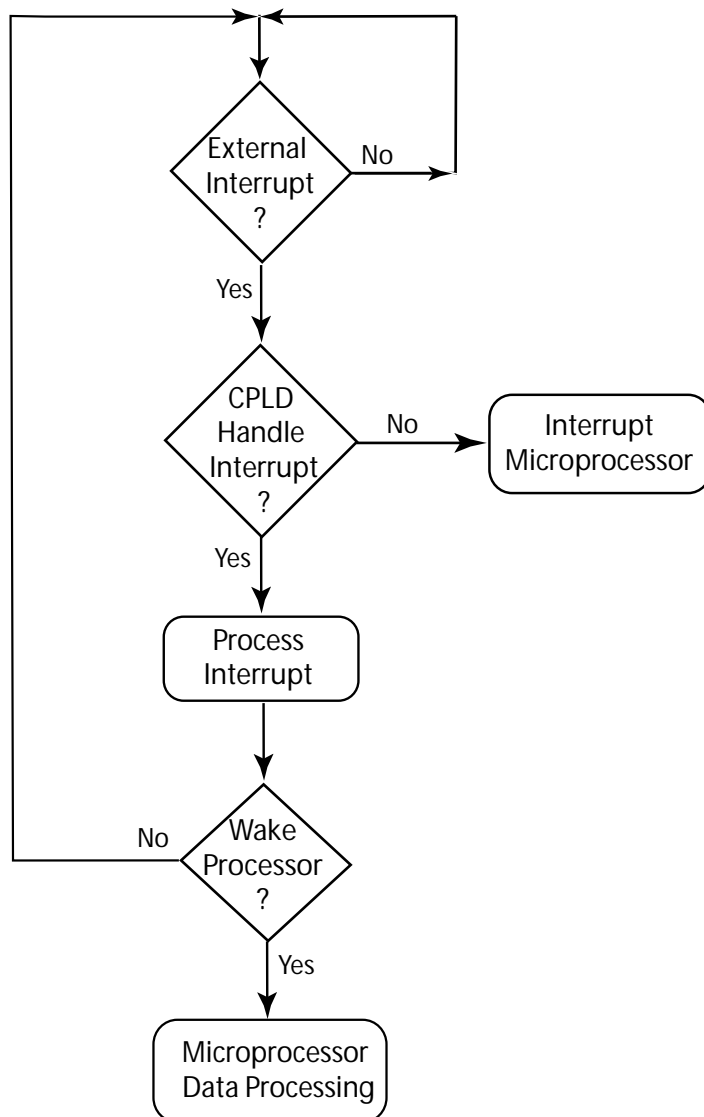
Figure 5: CPLD Flow Diagram
