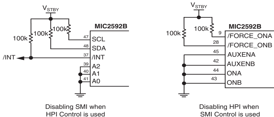
Figure 6. Input Pin Configuration for Disabling HPI/SMI Control
