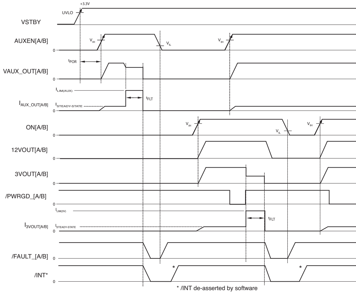
Figure 8. Hot-Plug Interface Operation
