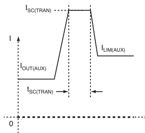
Figure 5. VAUX Current Limit Response Timing
