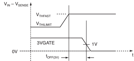
Figure 3. 3V Current Limit Response Timing
