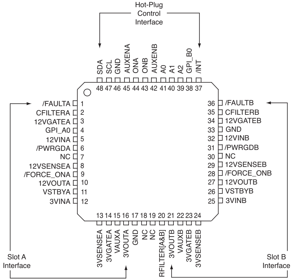
48-Pin TQFP
