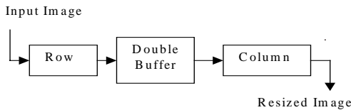
Figure 4 Resize Architecture
