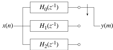
Figure 2 Polyphase Interpolator
