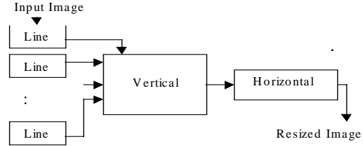
Figure 5 Zero Frame Latency Resizing
