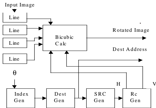
Figure 6 Rotation Architecture
