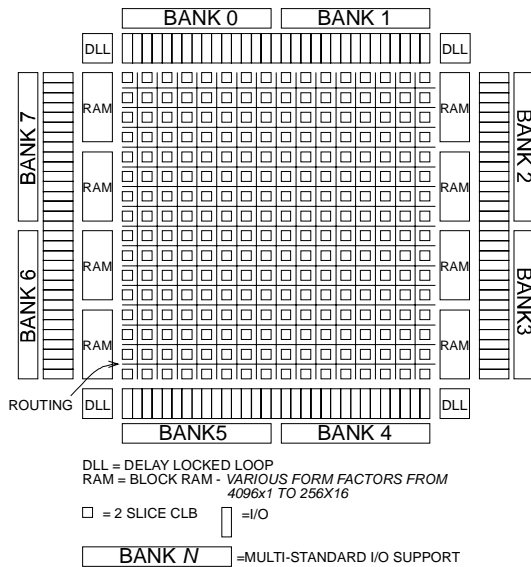
Figure 7 Xilinx Virtex FPGA Architecture
