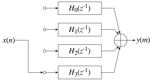
Figure 1 Polyphase Decimator
