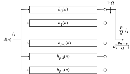
Figure 3 Polyphase Resampling
