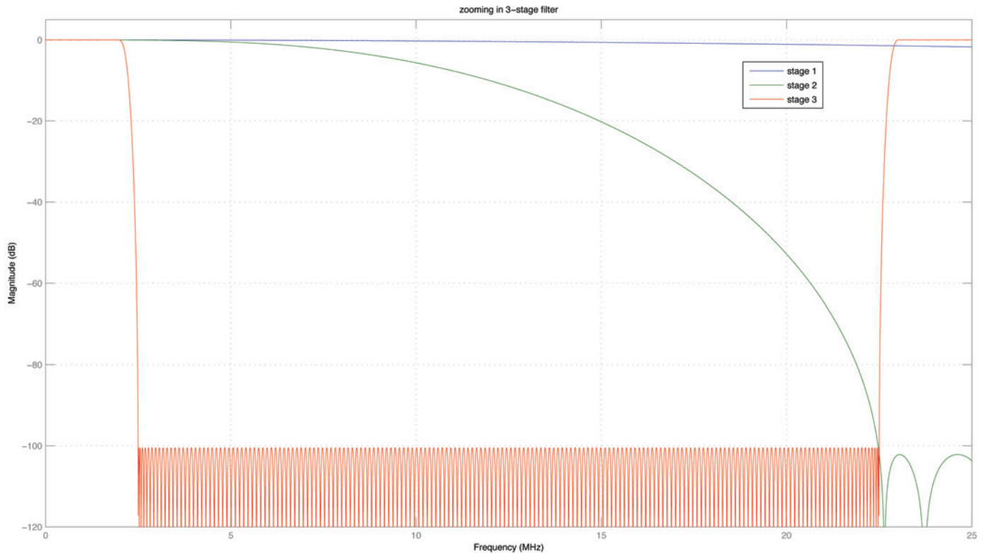
Figure 3 – Decimation by 50 via the cascade of three FIR filtering stages, here shown separately with a zoom in the frequencies from 0 to 25 MHz.
