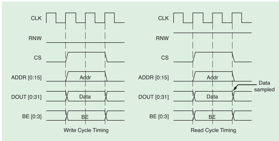
Figure 2 – A simple address-mapped user interface is synchronous to the clock.
