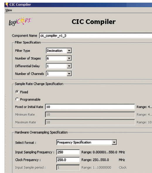
Figure 4 – Settings for the CIC filter decimating by 10. Page 1/3 of CIC-Compiler 1.3 GUI.
