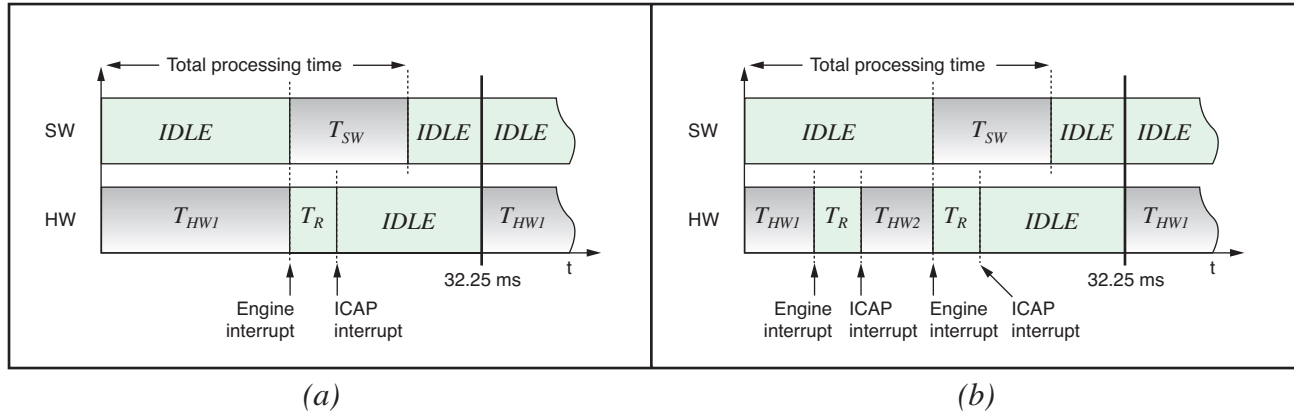
Figure 1 – Depending on the number of reconfigurations and when they are performed, the process is either inter- or intra-video frame reconfiguration, or InterVFR (a) and IntraVFR (b).
