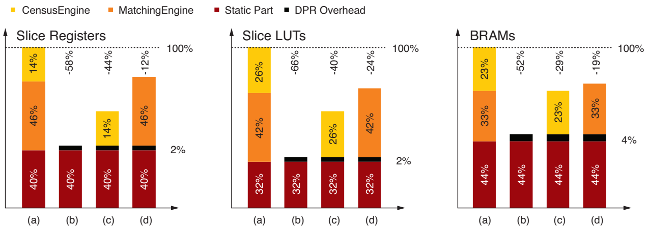
Figure 5 – Worst-case resource saving of a reconfigurable vs. a nonreconfigurable system
