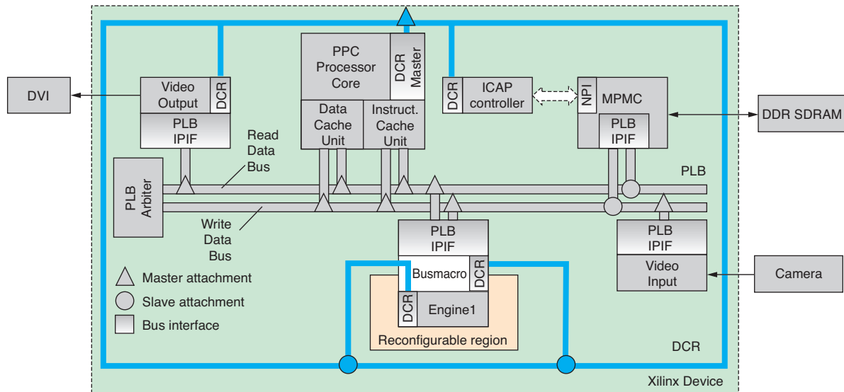
Figure 2 – Block diagram of the AutoVision system shows how the ICAP controller links to MPMC via a Native Port Interface.
