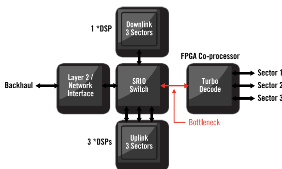
Figure 1: Traditional 3G co-processor architectures do not scale to the increased demands of 4G
