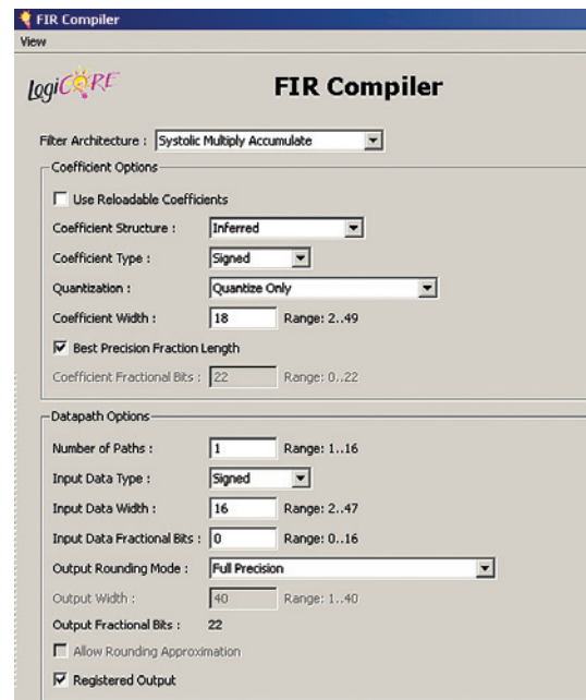
Figure 2 – Integer downsampling by 50. Page 2/4 of FIR-Compiler 5.0 GUI settings for the reference single-stage filter.
