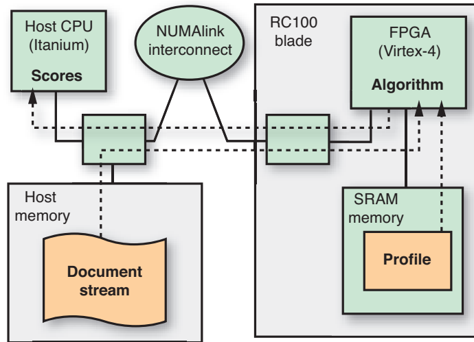
Figure 2 – In the FPGA subsystem architecture, Virtex-4 devices connect to the host platform via SGI's NUMalink interface.
