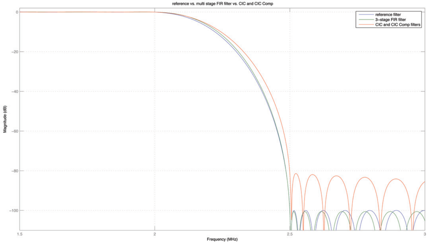
Figure 5 – Frequency responses of the three downsamplers with overall rate change of 50 and with zoom in the frequency range from 1.5 to 3 MHz. The single stage is shown in blue, the three-stage (ratios M1=2 , M2=5 , M3=5 ) is in green and the two-stage CIC-based (ratio M1=10 , M2=5 ) is in red.
