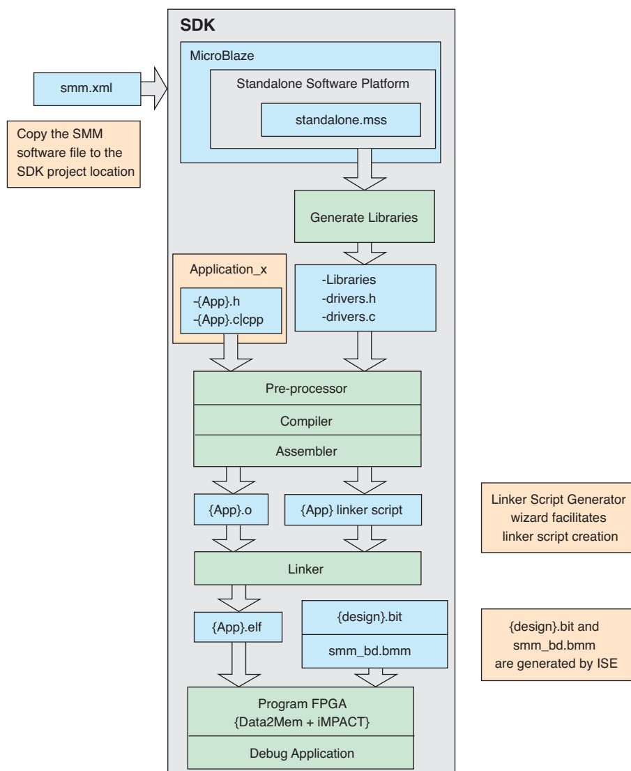
Figure 4 – The SDK development flow starts with the software definition file.
