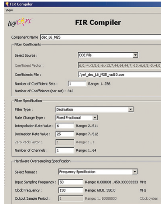
Figure 6 – Rational downsampling by 25/6. Page 1/4 of FIR-Compiler 5.0 GUI settings for the reference single-stage filter.
