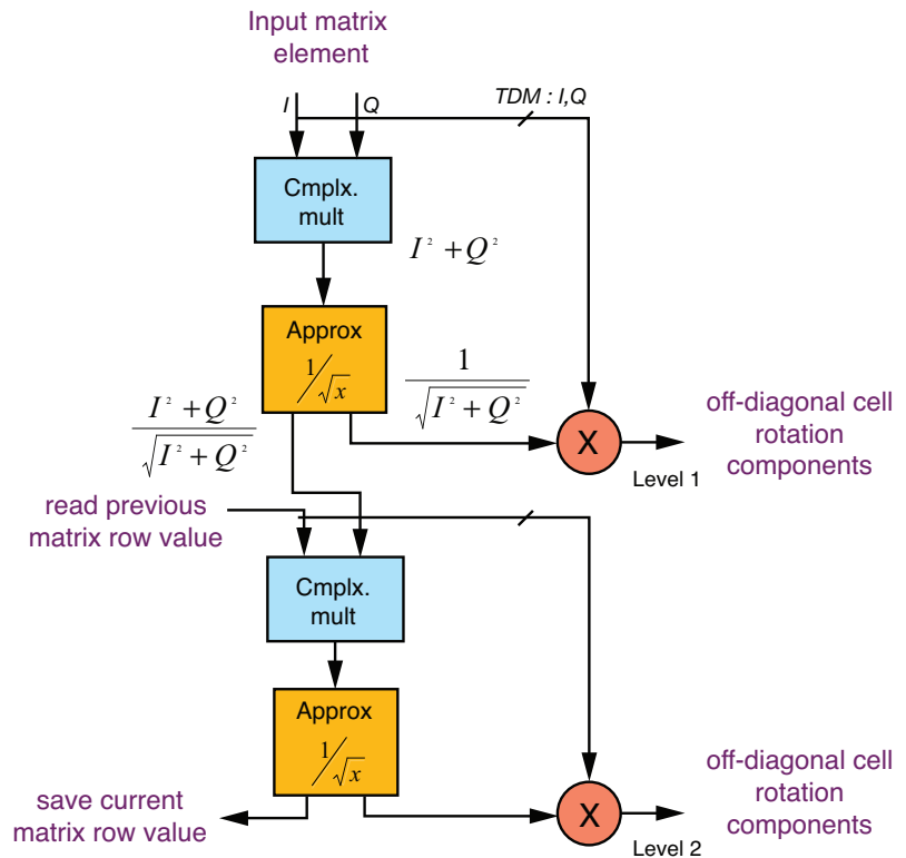
Figure 3 – Block diagram of the diagonal systolic-array cell
