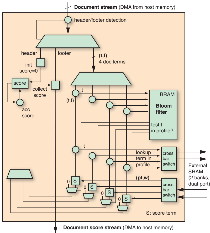
Figure 3 – Diagram of FPGA implementation of a filtering application
