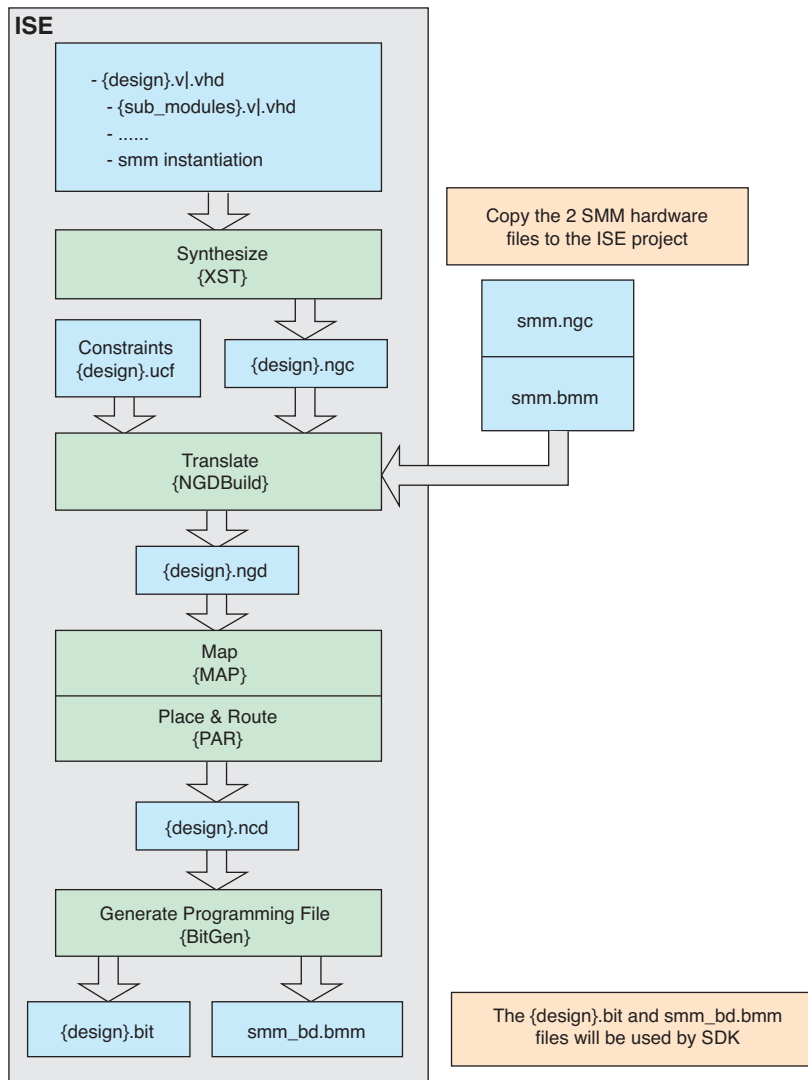
Figure 3 – The FPGA design flow follows the standard ISE FPGA implementation flow, with no need for new tools or scripts.
