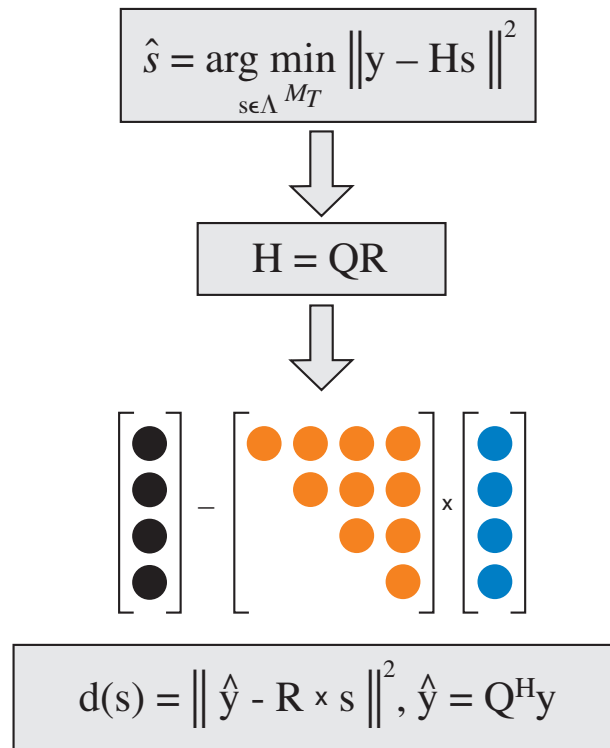
Figure 1 — Partial Euclidian distance metric equation for sphere detector-based MIMO detection
