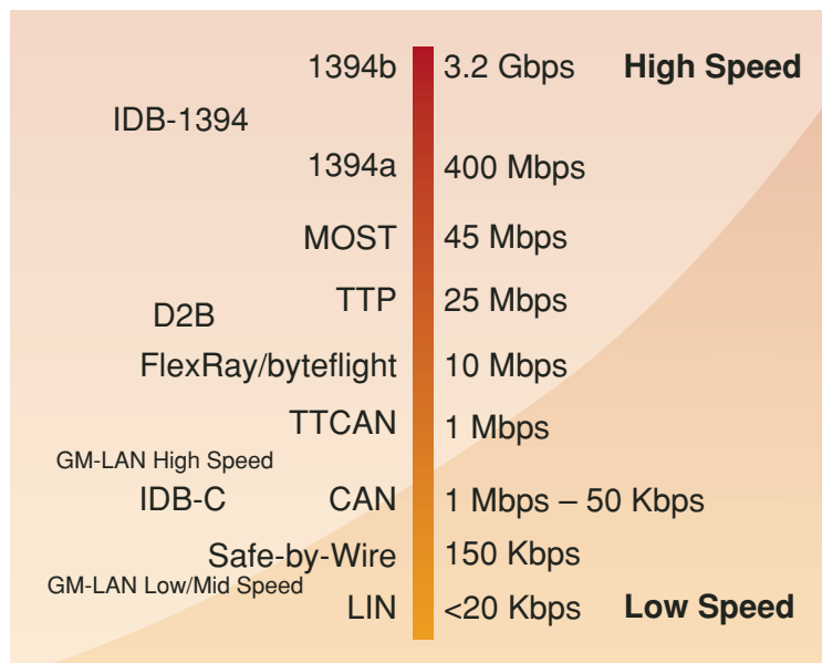
Figure 1 – In-car network data-transfer speeds
