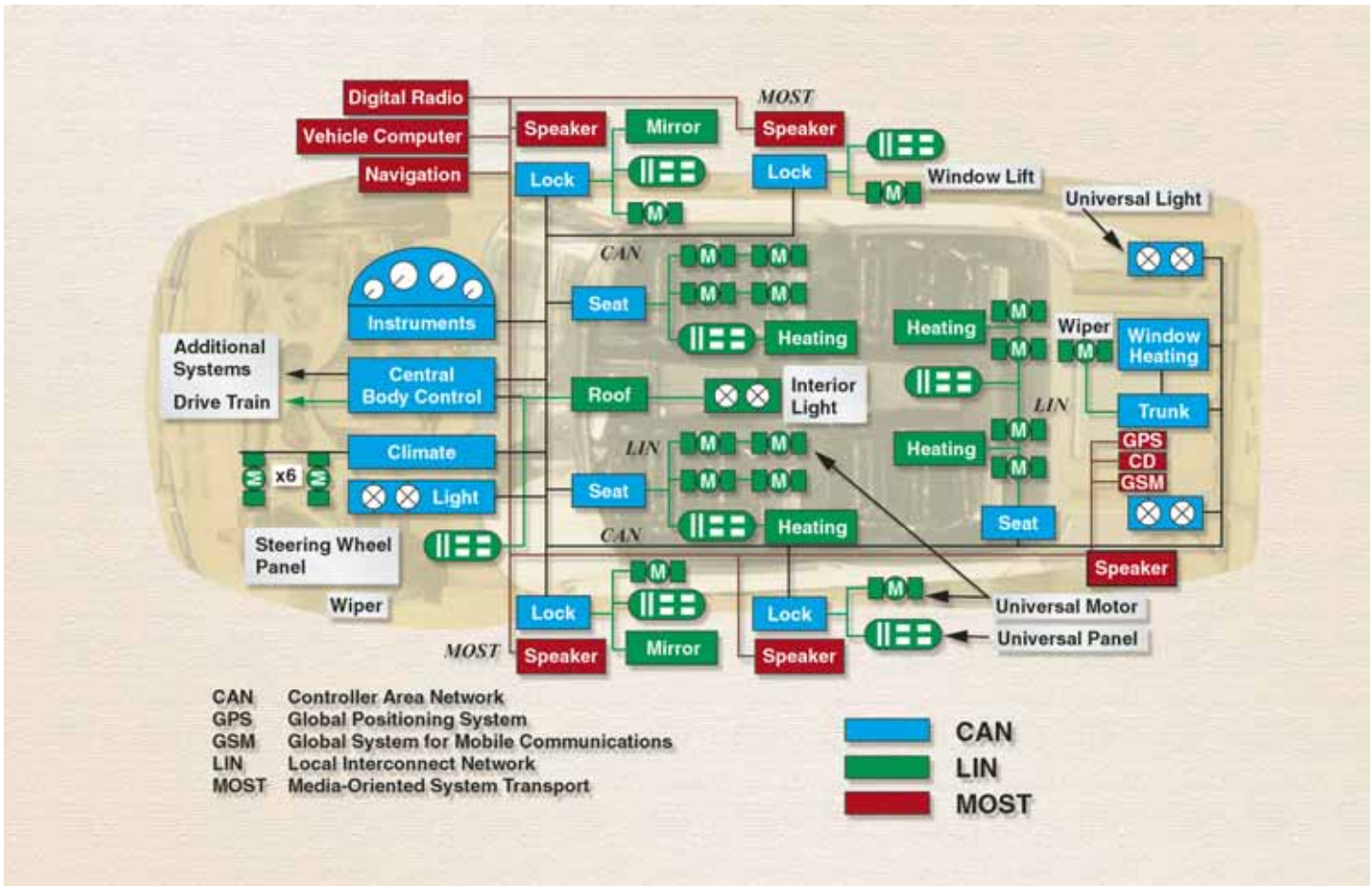
Figure 3 – In-car complementary networks
