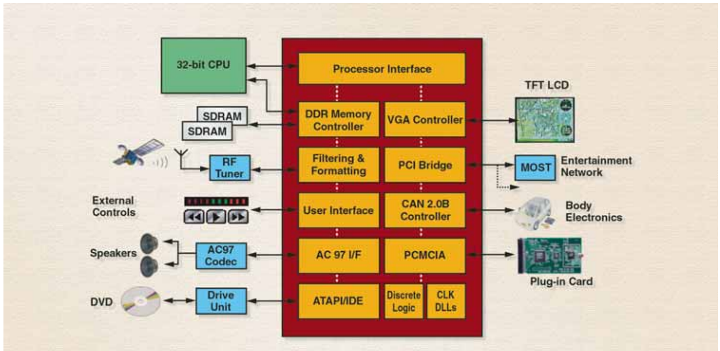
Figure 2 – In-car multimedia functions embedded in an FPGA
