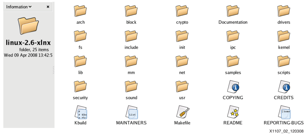
Figure 2: linux-2.6-xlnx Directory
