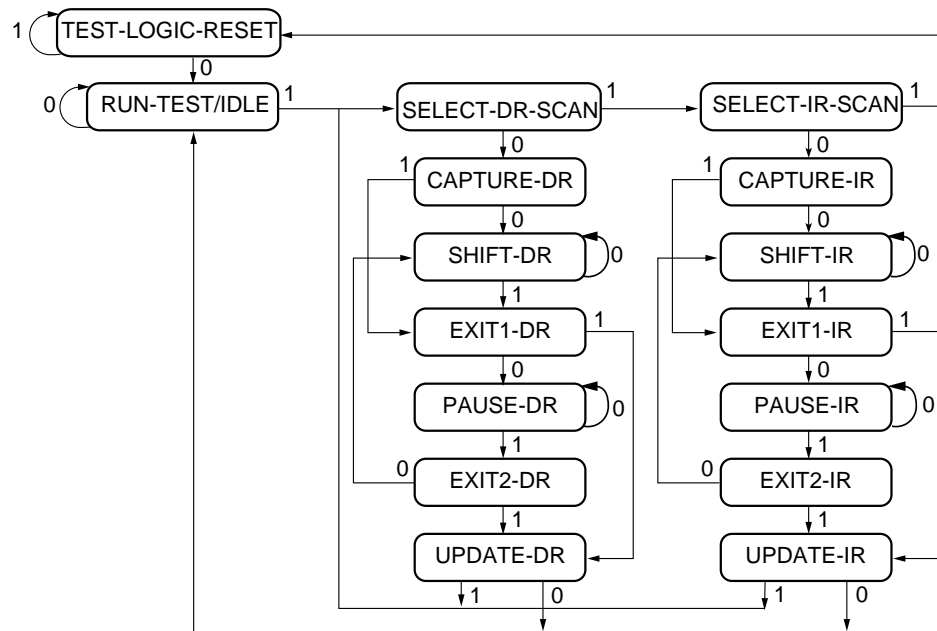
Figure 1: State Diagram for the TAP Controller
