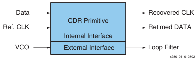
Figure 1: CDR Primitive
