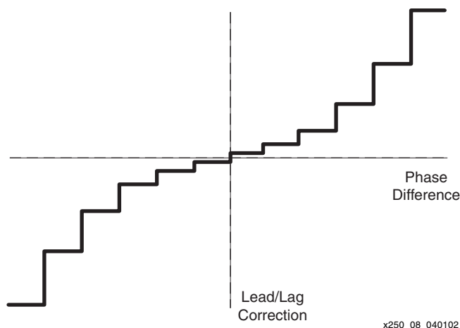
Figure 8: Phase Error Output
