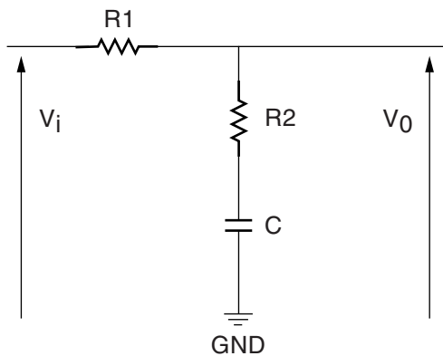
Figure 11: Loop Filter
