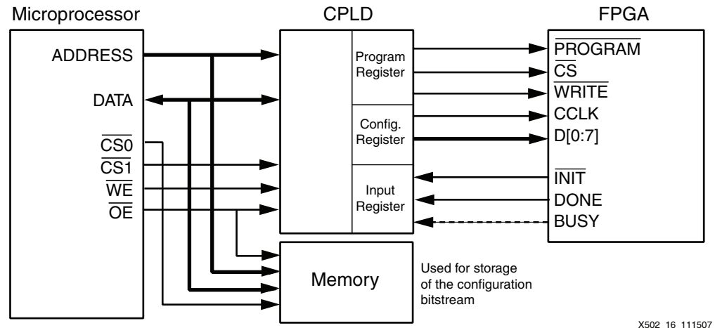
Figure 6: SelectMAP Configuration
