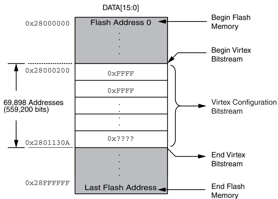
Figure 5: Flash Memory Map
