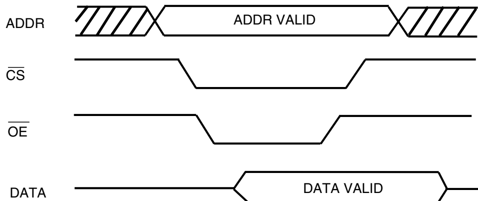
Figure 13: Read-Cycle Timing Diagram
