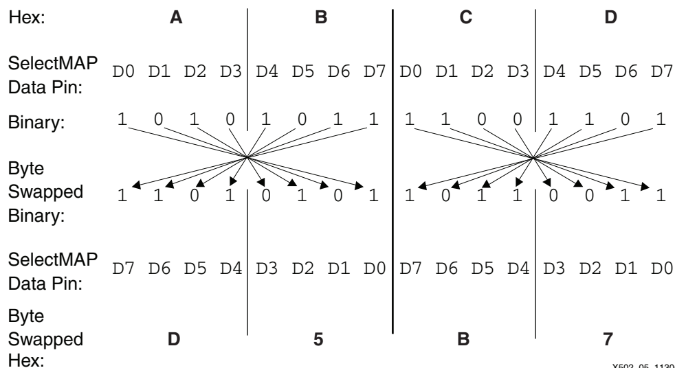
Figure 3: Byte-Swapping Example
