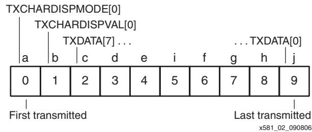
Figure 2: 10-bit TX Data Map with 8B/10B Bypassed
