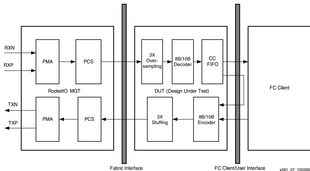
Figure 7: Far-End Loopback Test Setup
