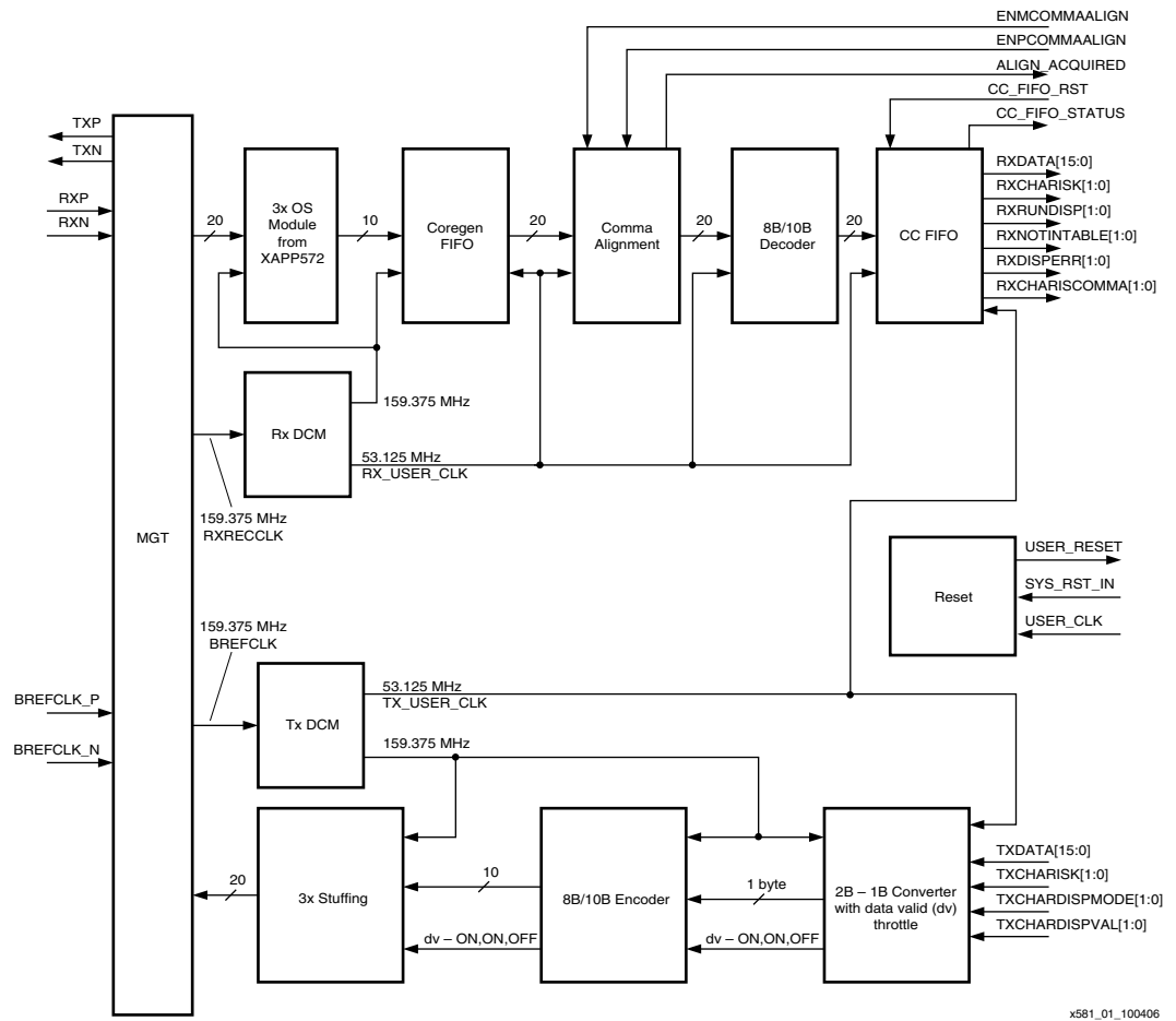
Figure 1: RocketIO 3X-Oversampling Reference Design Block Diagram
