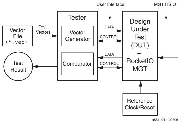
Figure 4: Simulation Testbench
