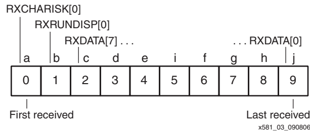
Figure 3: 10-bit RX Data Map with 8B/10B Bypassed
