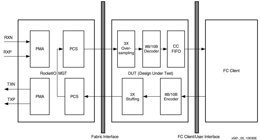
Figure 5: Parallel Loopback Test Setup
