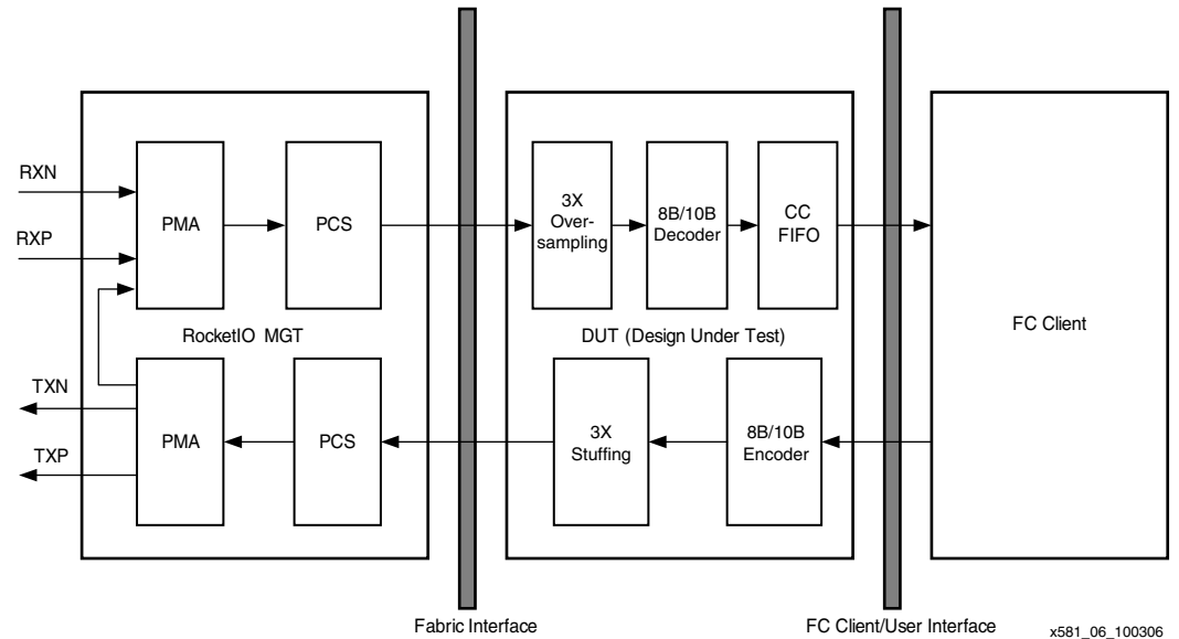
Figure 6: Serial Loopback Test Setup
