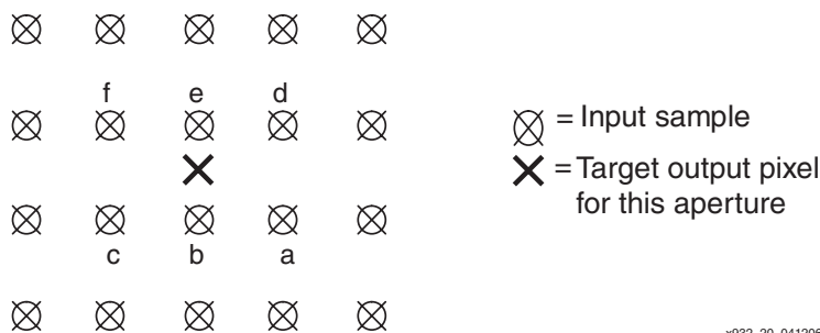
Figure 20: 4:4:4 to 4:2:0 Coefficient Configuration
