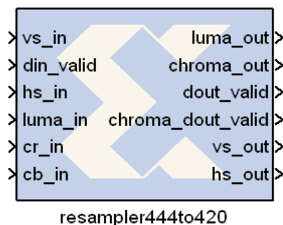
Figure 19: Convert444to420 Block
