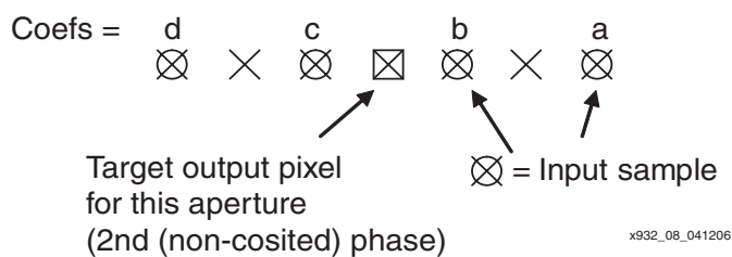
Figure 9: 4:2:2 to 4:4:4 Coefficient Configuration
