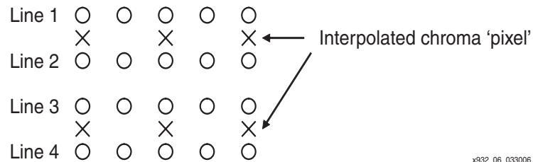
Figure 6: 4:2:0 Graphical Representation
