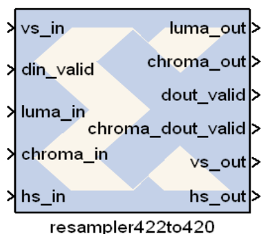
Figure 14: Convert422to420 Block
