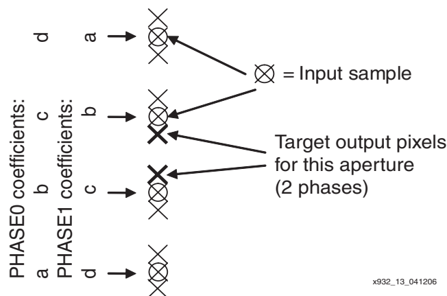
Figure 13: 4:4:4 to 4:2:2 Coefficient Configuration
