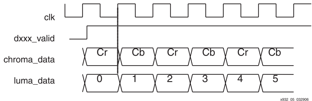
Figure 5: 4:2:2 Delivery Format
