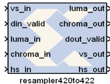
Figure 12: Convert420to422 Block
