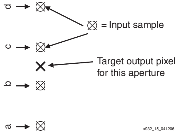
Figure 15: 4:2:2 to 4:2:0 Coefficient Configuration
