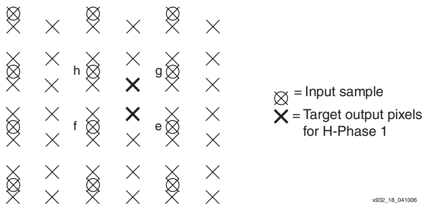
Figure 18: 4:4:4 to 4:2:0 Coefficient Configuration (H-phase 1)
