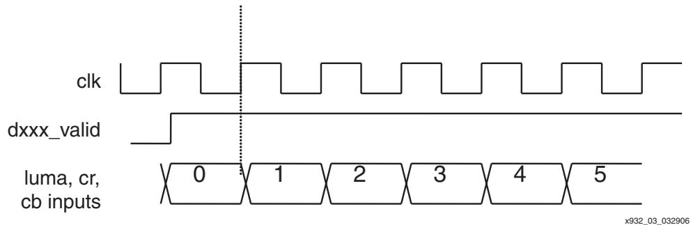
Figure 3: 4:4:4 Graphical Representation
