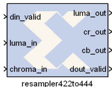
Figure 8: Convert422to444 Block
