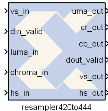
Figure 16: Convert420to444 Block
