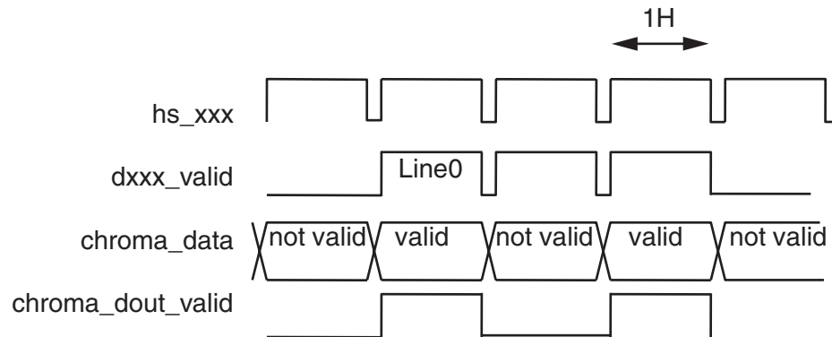
Figure 7: 4:2:0 Delivery Format
