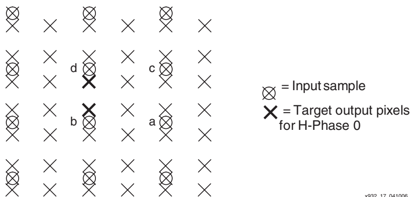
Figure 17: 4:2:0 to 4:4:4 Coefficient Configuration (H-phase 0)
