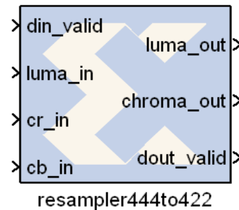
Figure 10: Convert444to422 Block
