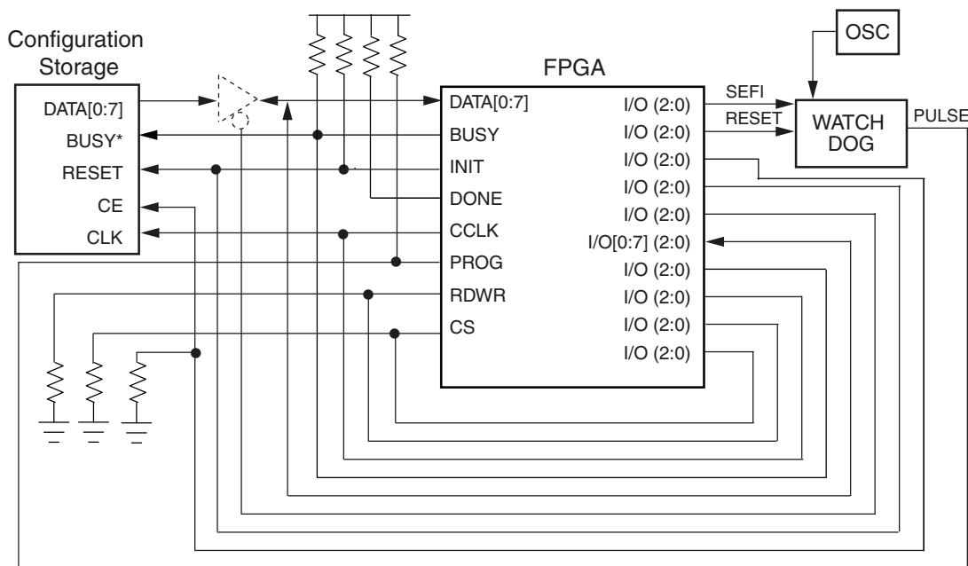
Figure 2: Overview of single FPGA, in Master SelectMAP Mode, Self-Hosting a Triplicated Configuration Management
