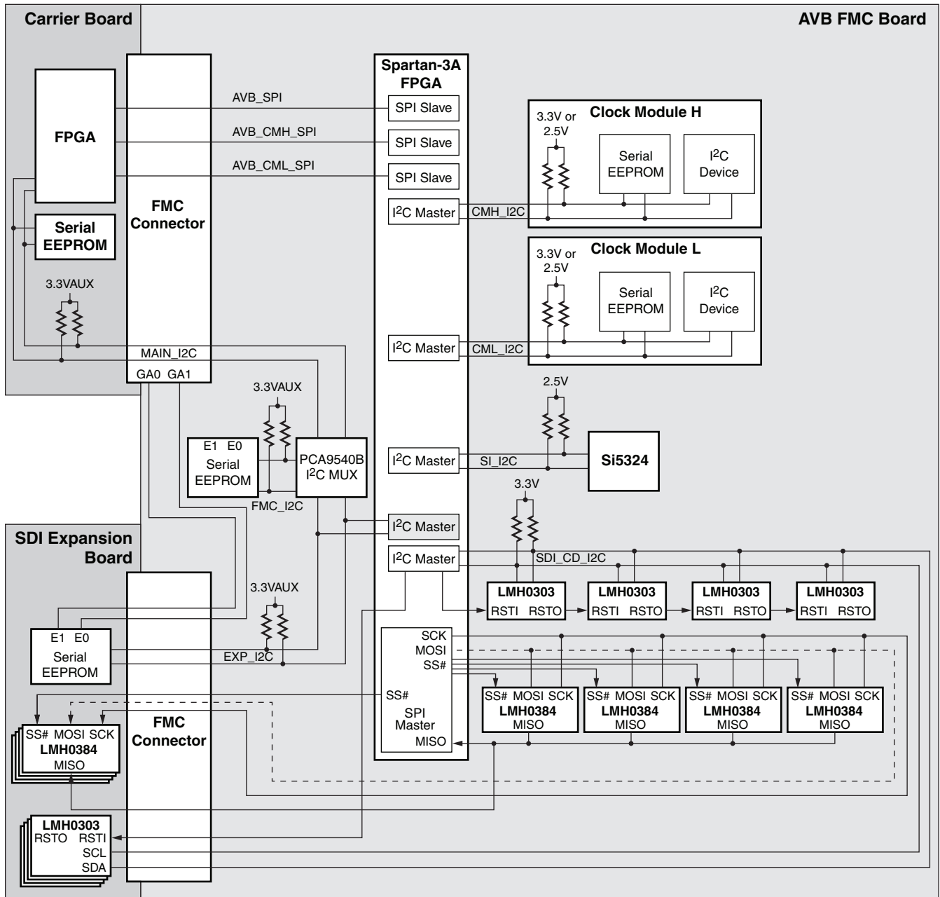
Figure 3: I2C and SPI Interfaces
