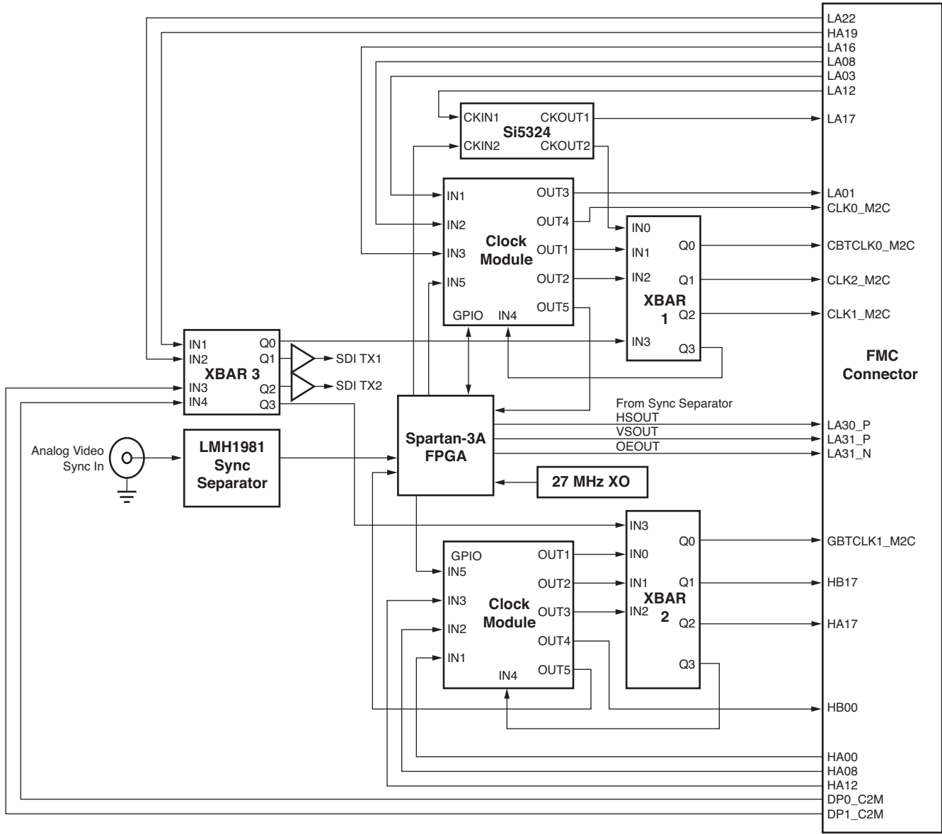
Figure 2: Clock Paths Block Diagram
