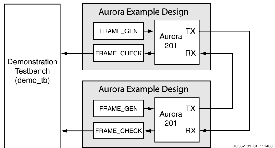
Figure 3-2: Example Design
