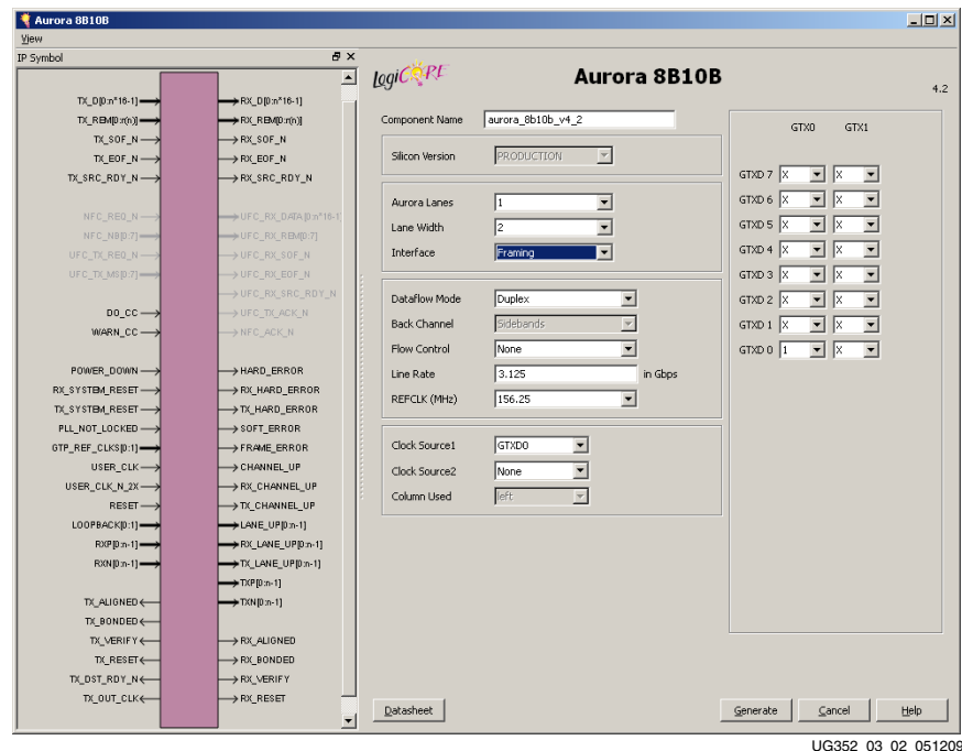
Figure 3-4: CORE Generator Aurora 8B/10B Customization Screen
