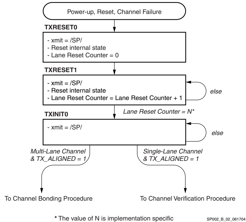
Figure B-2: Transmit Interface Lane Initialization Procedure
