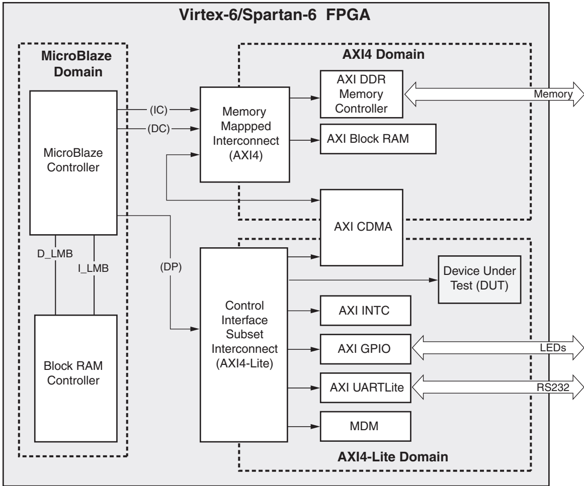
Figure 16: Virtex-6 and Spartan-6 FPGA System with the AXI HWICAP Core as the Device Under Test (DUT)
