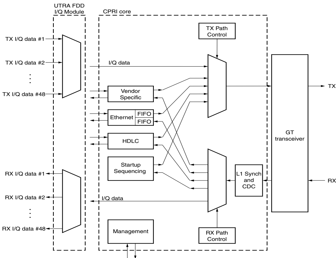
Figure 1: CPRI Top-Level Block Diagram
