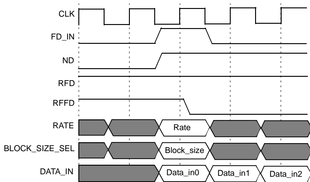
Figure 2: FD_IN Input With RFFD (ND Must Be High for FD_IN to be Valid)
