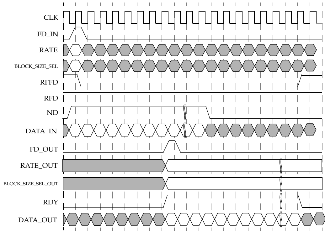
Figure 3: Control Signals on Data Input and Output
