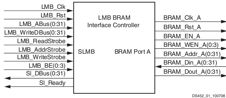
Figure 1: Dual LMB BRAM Interface Controller Block Diagram
