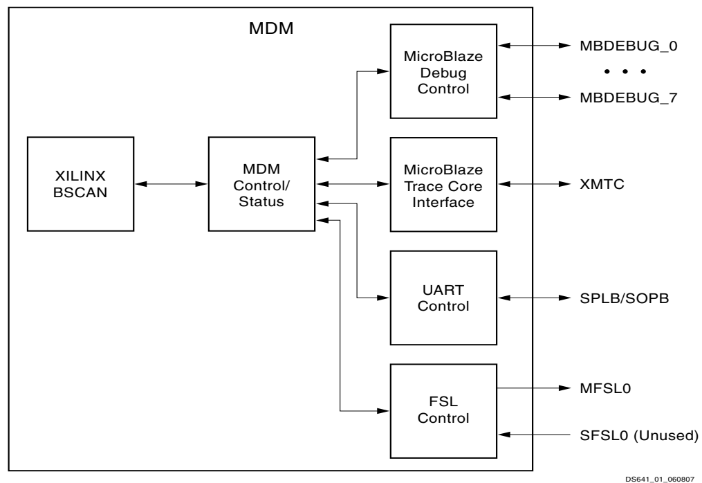
Figure 1: Microprocessor Debug Module (MDM) Block Diagram
