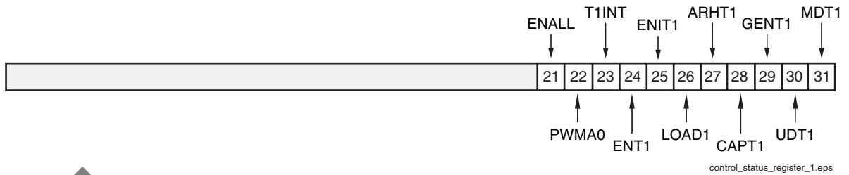
Figure 6: Timer/Status Control Register 1 (TCSR1)
