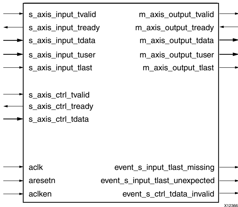
Figure 2-1: Core Schematic Symbol
