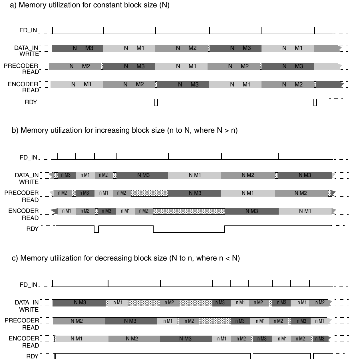
Figure 4: Triple-Buffering Memory Utilization
