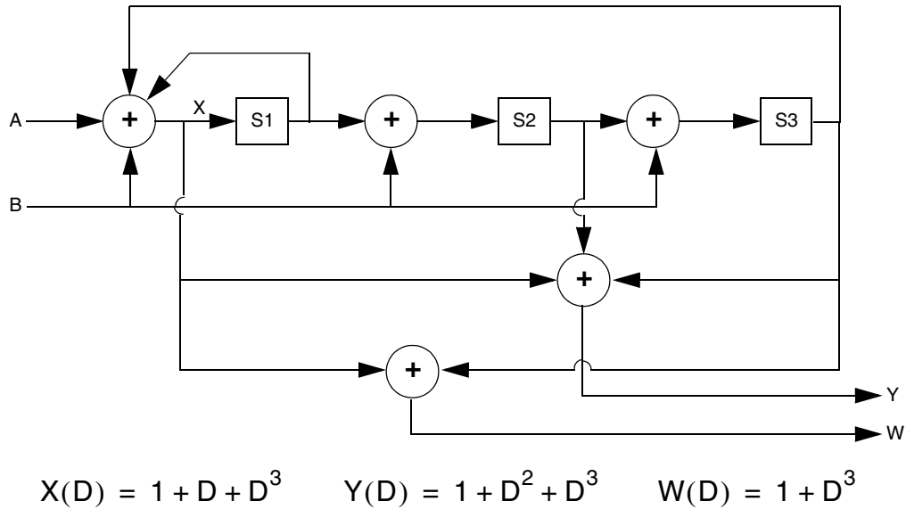
Figure 2: CRSC Constituent Encoder
