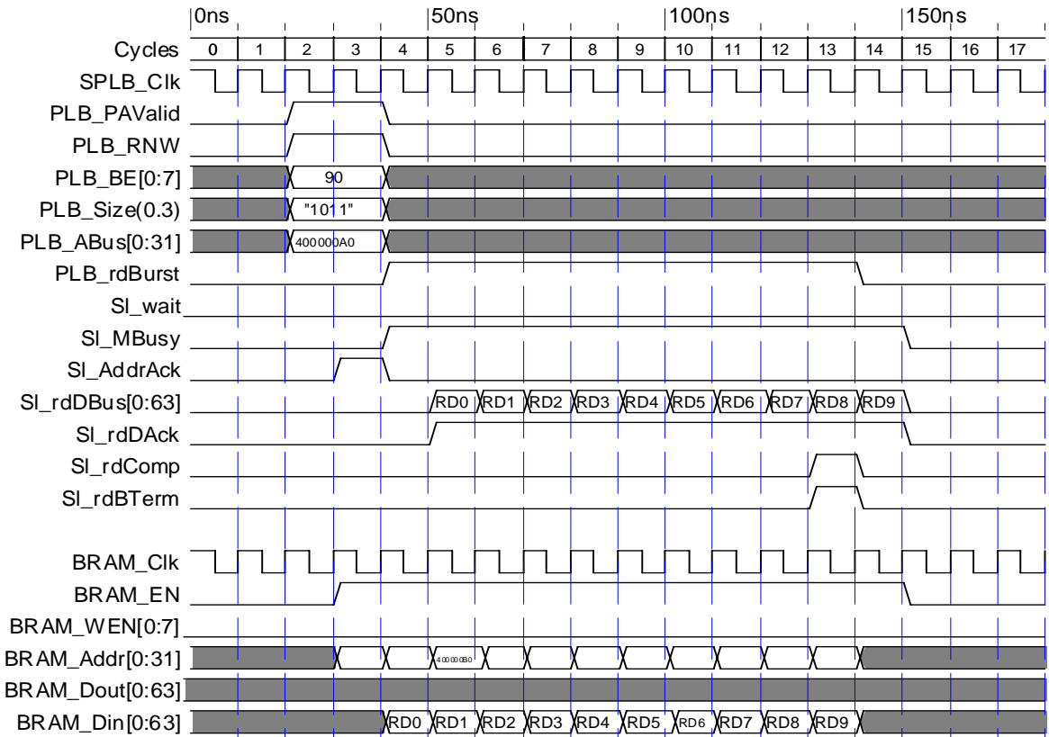
Figure 9: Fixed Length Burst Read (C_SPLB_SUPPORT_BURSTS = 1)
