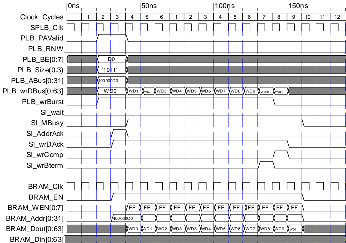
Figure 10: Fixed Length Burst Write (C_SPLB_SUPPORT_BURSTS = 1)
