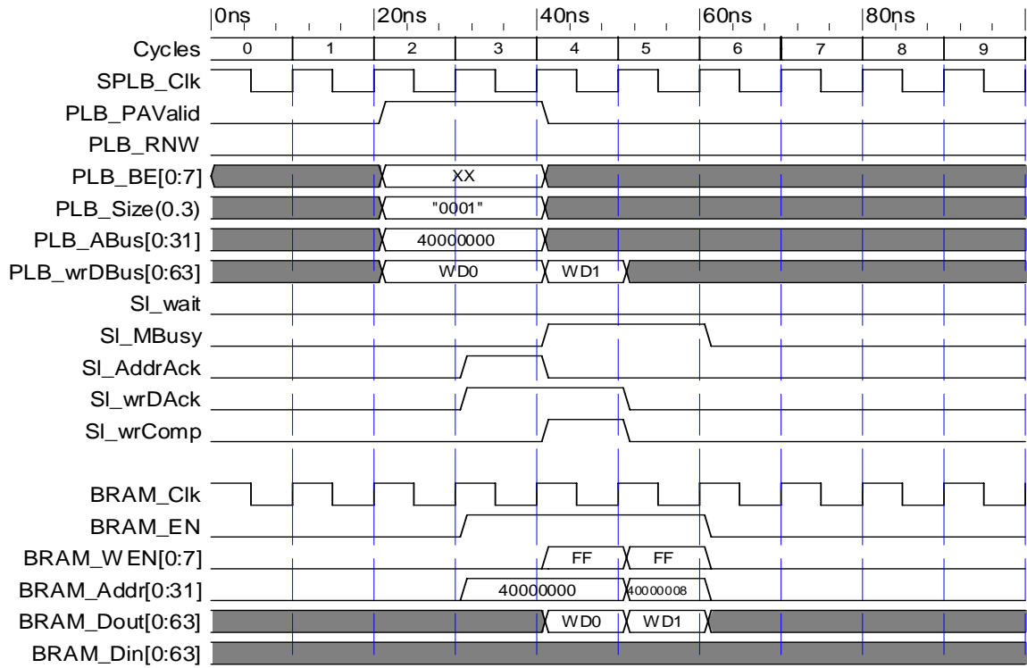
Figure 7: 4-Word Cacheline Write (C_SPLB_SUPPORT_BURSTS = 1)
