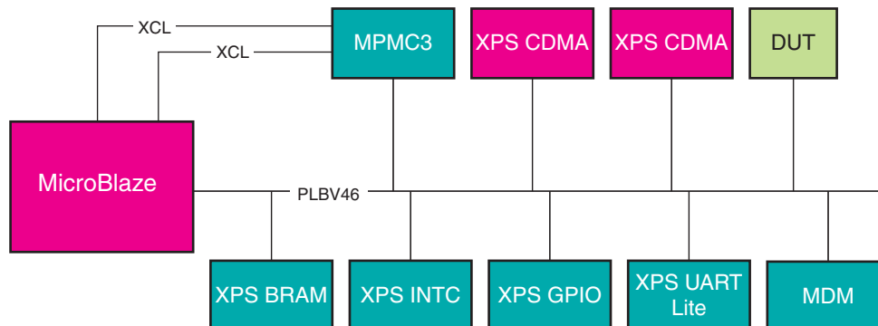
Figure 12: Virtex-5 LX System
