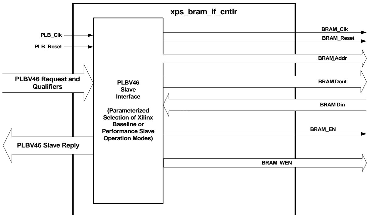
Figure 1: XPS BRAM Interface Controller Block Diagram
