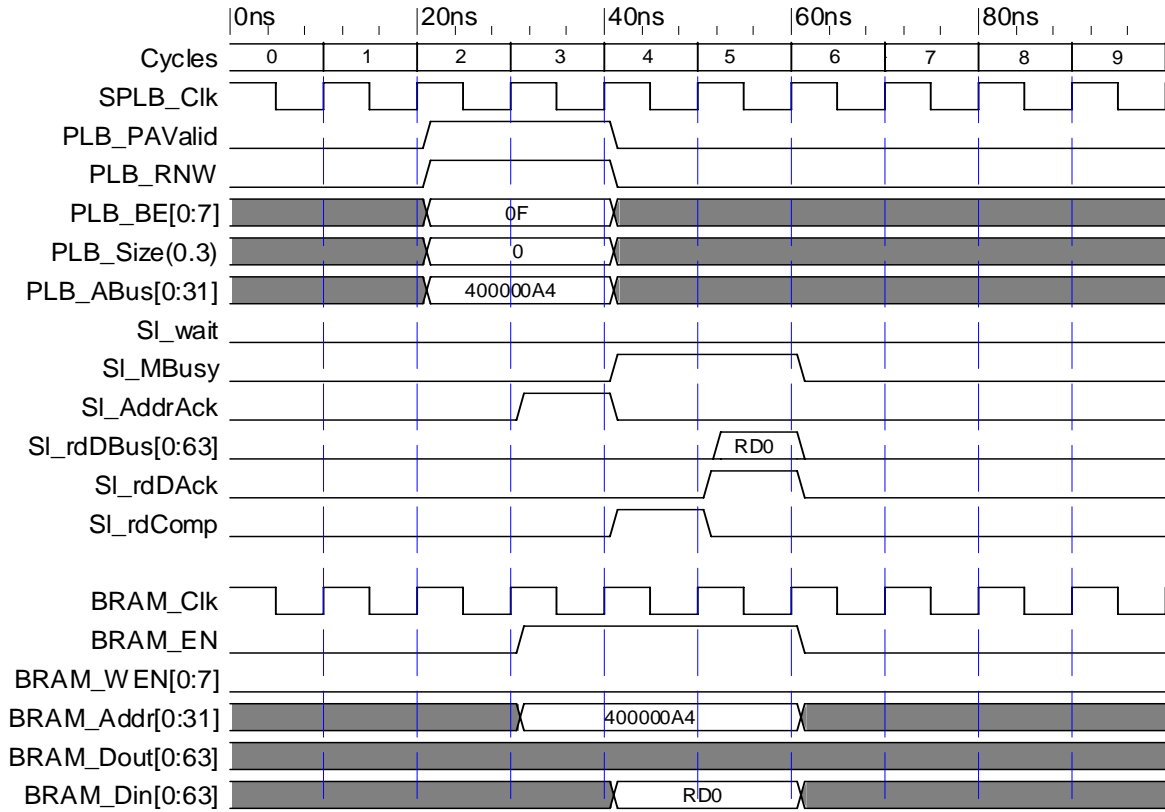
Figure 3: Single Data Beat Read
