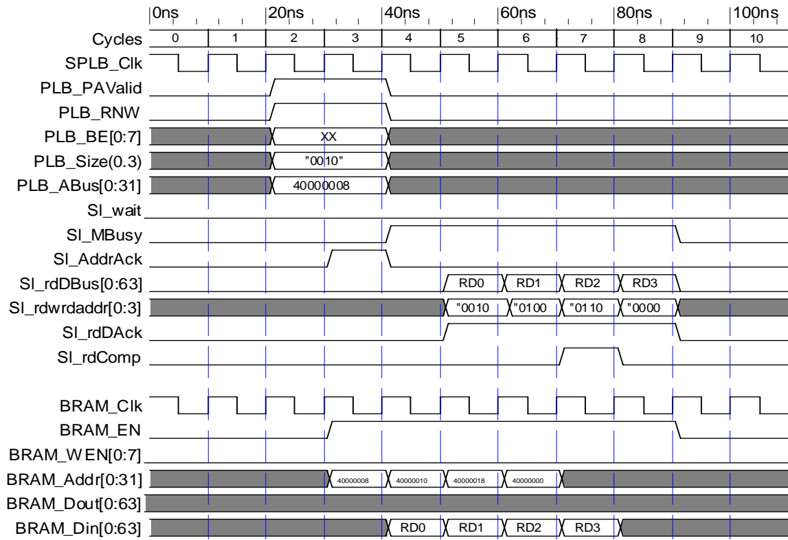
Figure 6: 8-Word Cacheline Read (C_SPLB_SUPPORT_BURSTS = 1)
