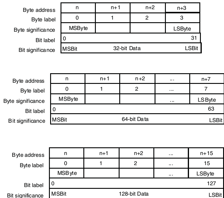
Figure 2: Big-Endian Byte Ordering and Left to Right Bit Numbering
