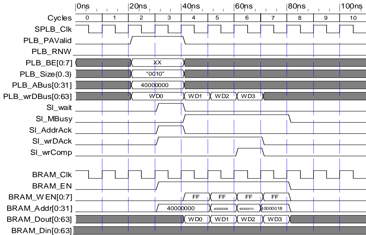
Figure 8: 8-Word Cacheline Write (C_SPLB_SUPPORT_BURSTS = 1)
