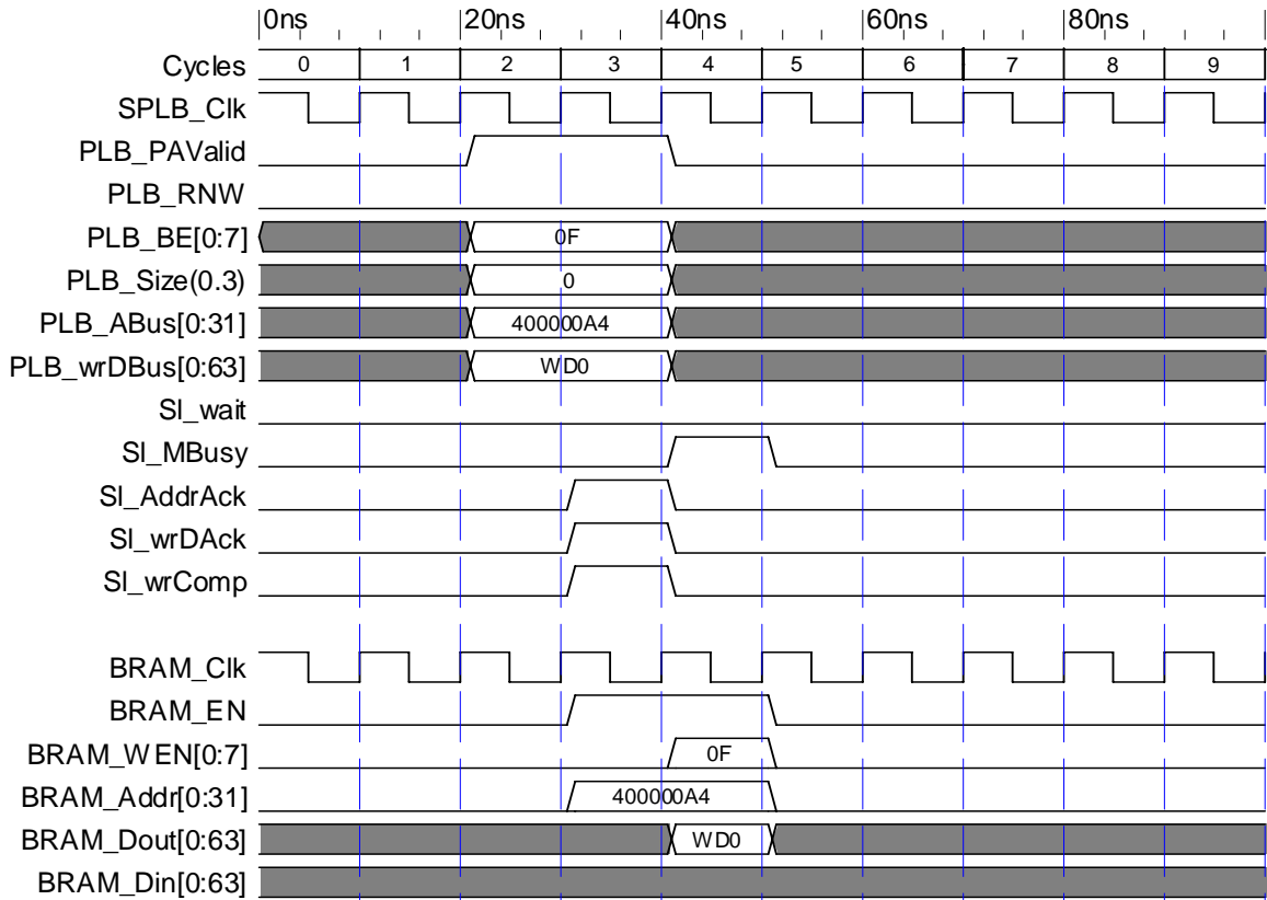
Figure 4: Single Data Beat Write
