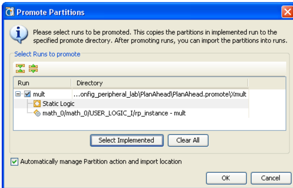
Figure 26: Promoting Partitions
