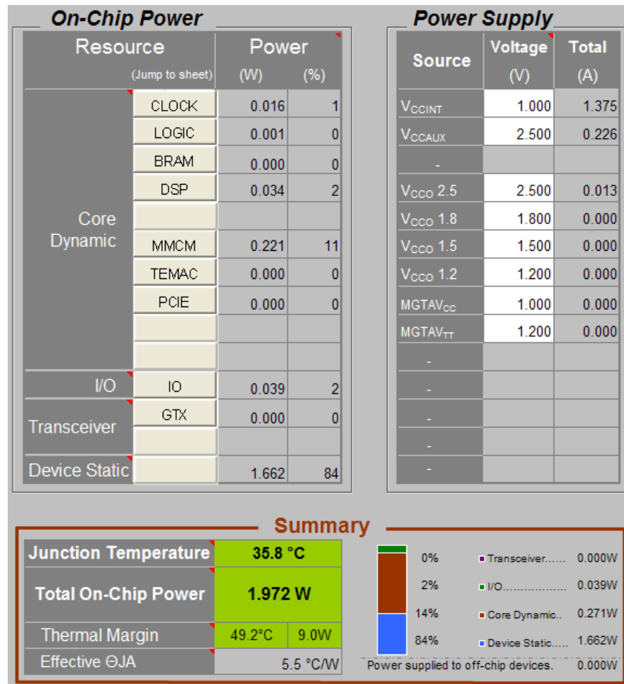
Figure 5: FPGA Power Summary - XPE for Virtex-6 FPGAs
