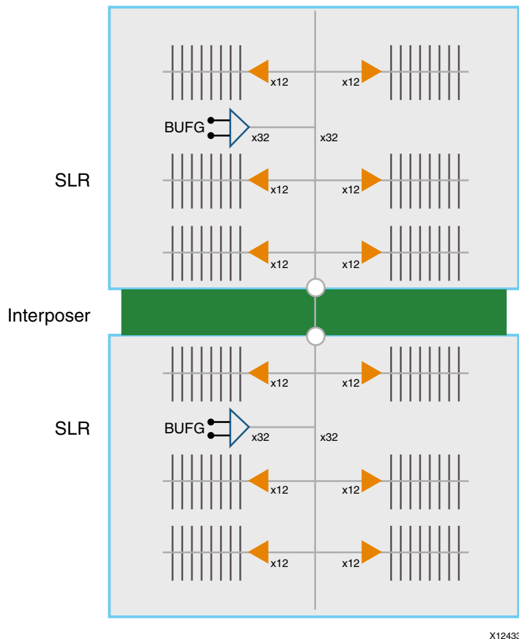
Figure 3-10: Global Clocking Connections in an SSI Device
