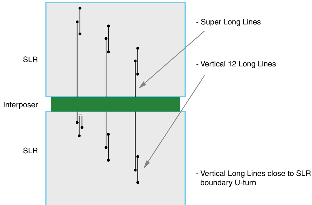
Figure 3-6: Representation of SLL Connectivity in the SLR
