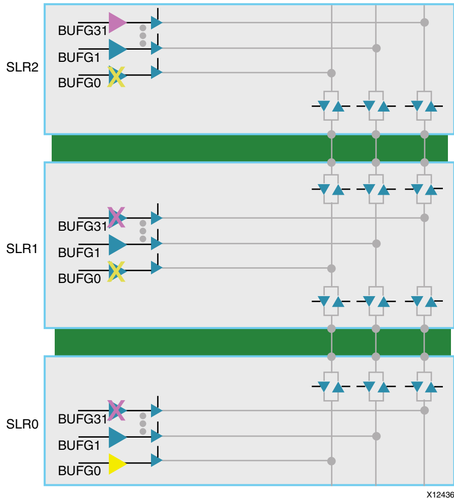
Figure 5-1: Clock Skew
