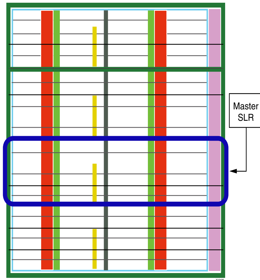
Figure 3-8: Master SLR in an xc7v2000t Device
