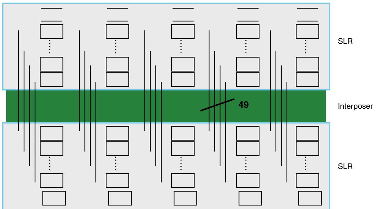
Figure 3-5: Staggered SLLS Crossing in an SSI Device
