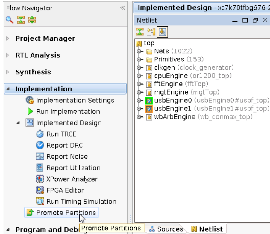
Figure 11: Promote Partitions
