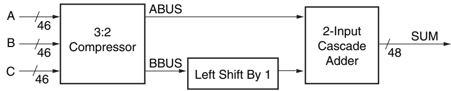
Figure 3-3: Three-Input Adder
