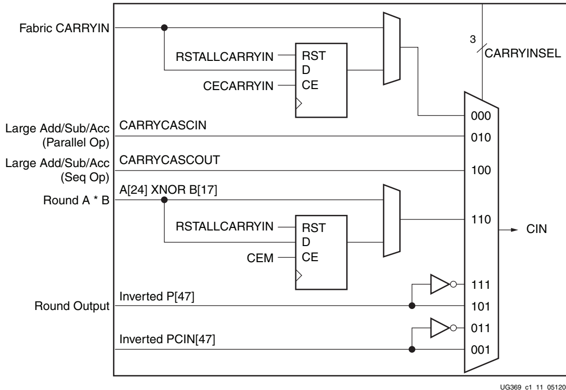
Figure 2-11: CARRYINSEL Port Logic
