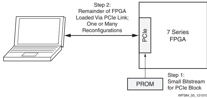
Figure 5: Partial Reconfiguration Tool Flow
