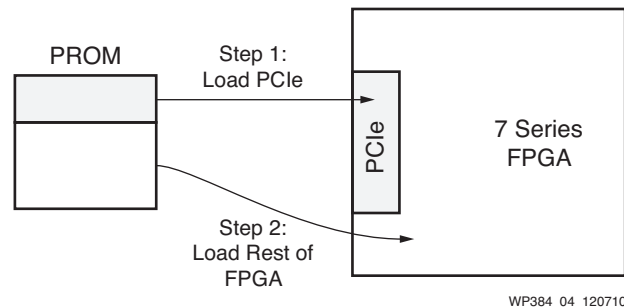
Figure 4: Two-Stage Bitstream Method
