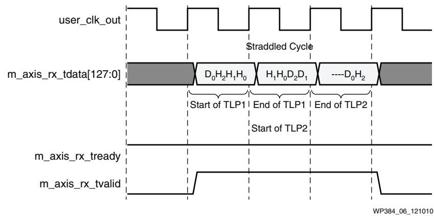
Figure 6: 7 Series Straddled Cycle
