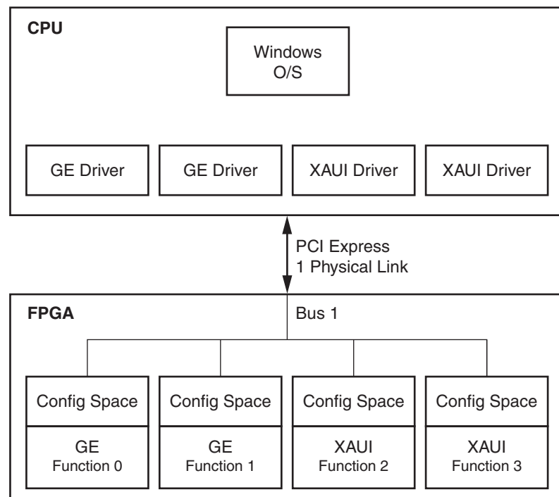
Figure 7: Multiple Function Devices
