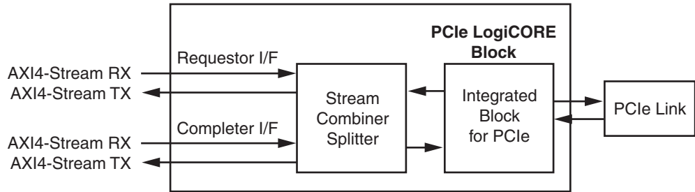
Figure 2: Enhanced AXI4-Stream Interface
