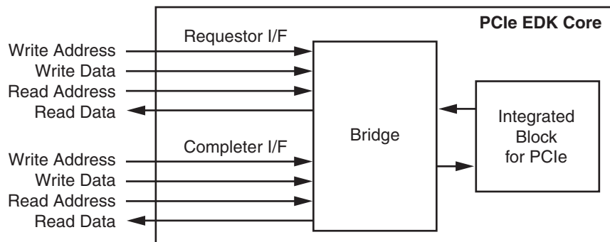
Figure 3: Basic AXI4 Interface
