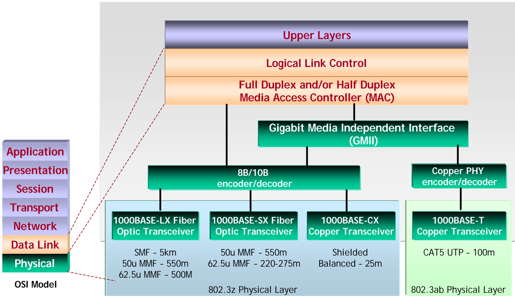
Gigabit Ethernet - Physical Structure
