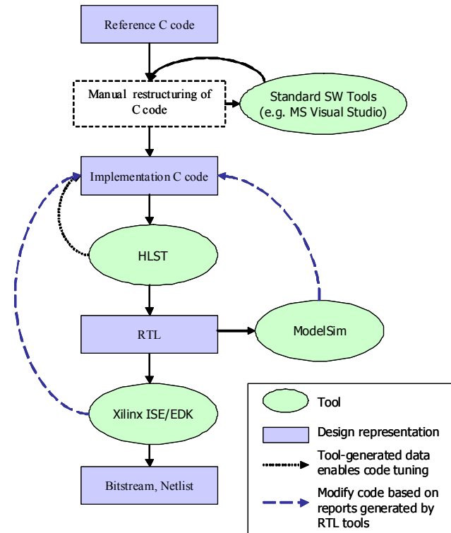
FIGURE 3. Design flow using the AutoPilot or PICO high-level synthesis tools in conjunction with Xilinx RTL tools. (Figure based on a diagram provided by AutoESL.)
