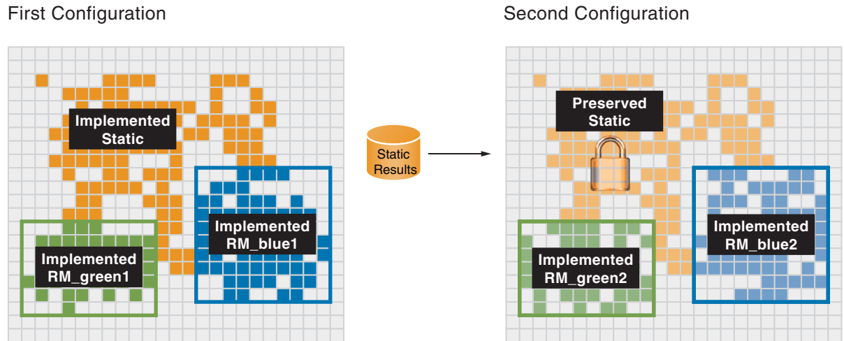
Figure 2: Partial Reconfiguration Design Flow
