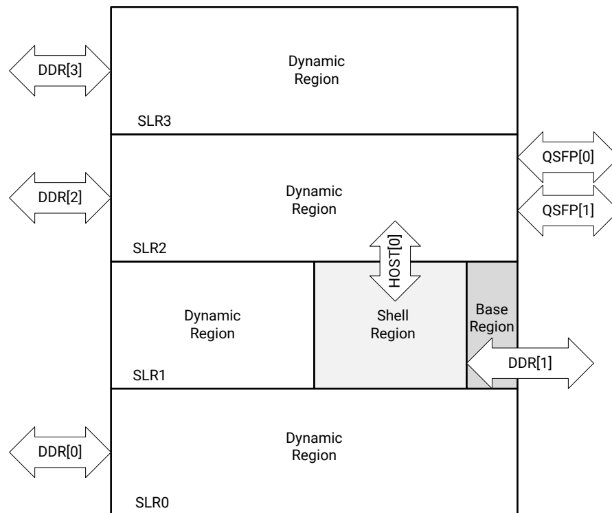
Figure 6: Floorplan
