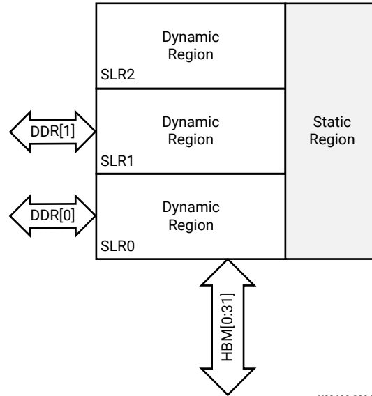
Figure 8: Floorplan
