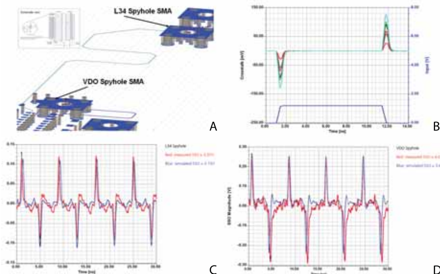
Figure 4 – Transient simulation results as computed by Nexxim: (a) simulation set-up and extracted S-parameters and IBIS drivers shown in schematic; (b) crosstalk caused by neighboring aggressors observed on victim pin; (c) measured results at L34 spy-hole compared to EM and transient simulation; (d) results at VDO spy hole.
