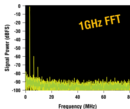
Undersampling a 1GHz Signal at 250Msps
