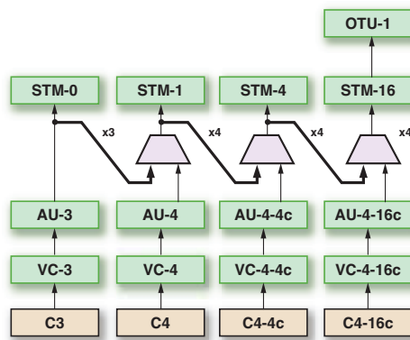
Figure 2 – SONET/SDH framing IP
