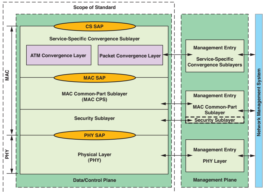
Figure 1 – The 802.16 protocol stack
