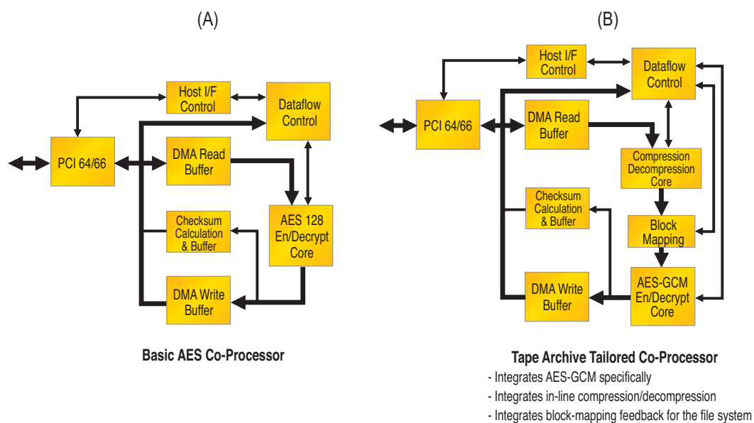
Figure 3 – A basic versus application-customized data security solution
