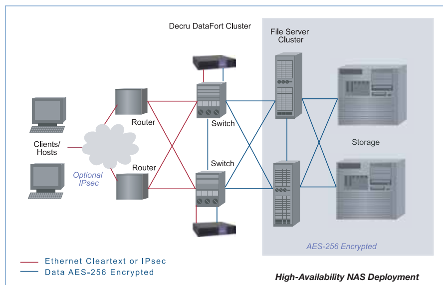
Figure 1 – High-availability deployment
