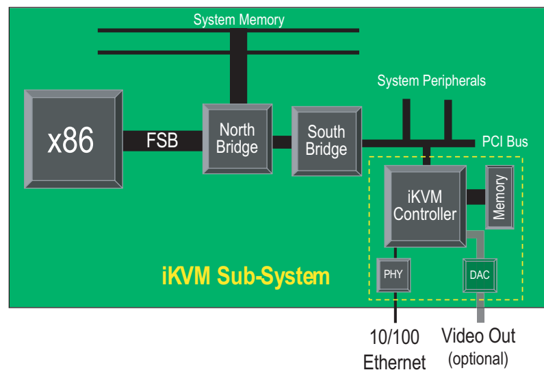
Figure 2 – Xilinx/Silicon Spectrum highly integrated iKVM platform
