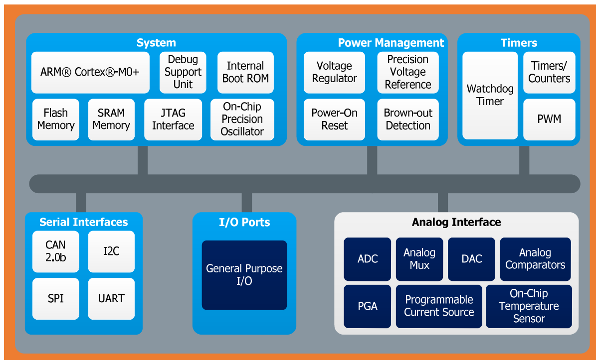
UT32M0R500 Block Diagram
