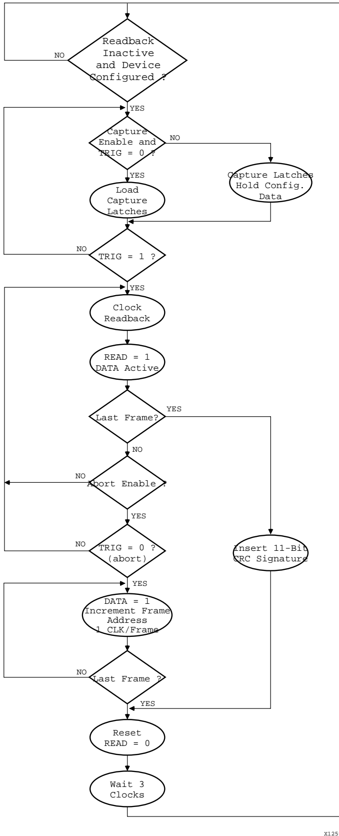
Figure 2. Readback State Diagram
