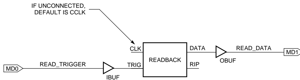
Figure 4. Readback Symbol on the Design Schematic
