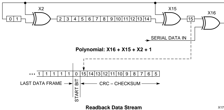
Figure 9. Circuit for Generating the CRC-16
