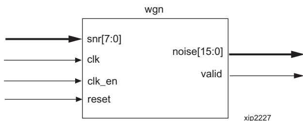
Figure 1: Core Schematic Symbol
