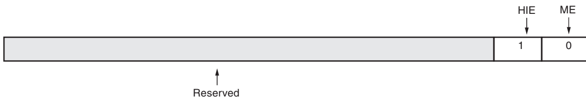
Figure 11: Master Enable Register (MER)
