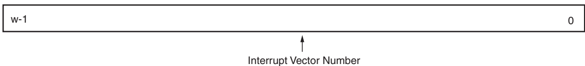
Figure 12: Interrupt Mode Register (IMR)
