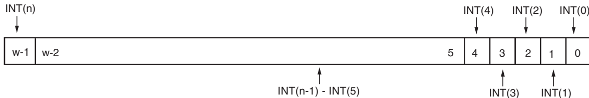
Figure 8: Set Interrupt Enable (SIE) Register
