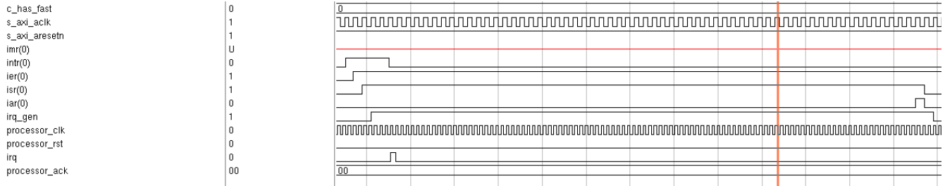
Figure 17: Input Intr - Level Sensitive (High), Output Irq - Edge Sensitive (Rising), C_HAS_FAST = 0
