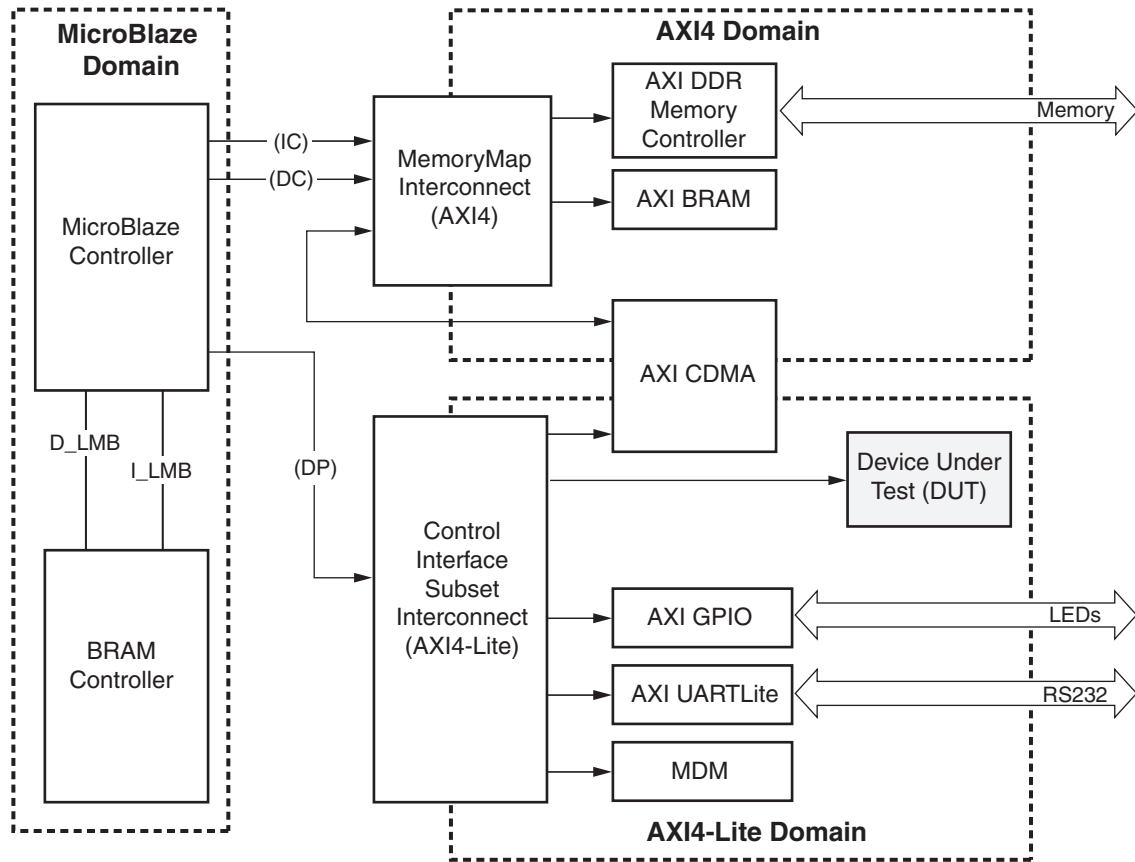
Figure 20: Virtex-6 and Spartan-6 Devices F MAX Margin System
