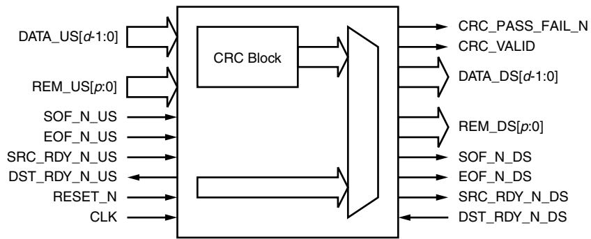
Figure 4: RX_CRC Module
