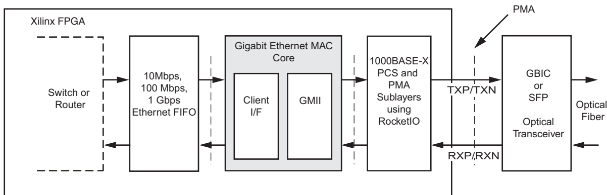
Figure 1: Typical GEMAC 1000BASE-X Application
