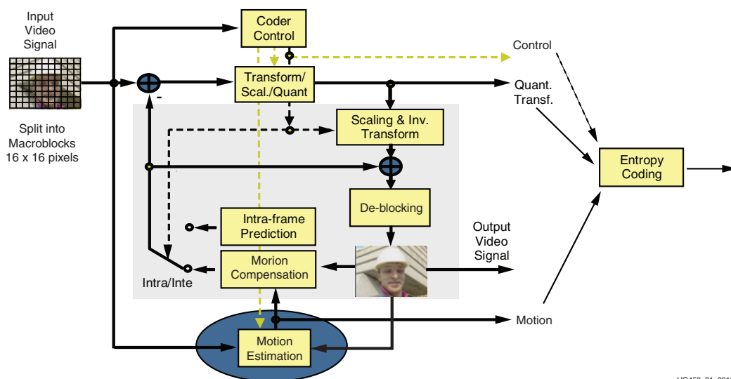
Figure 3-1: H.264 Encoder
