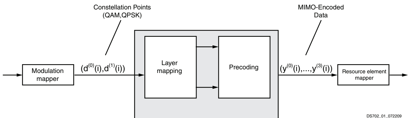
Figure 1: LTE MIMO Encoder v2.0 Functionality
