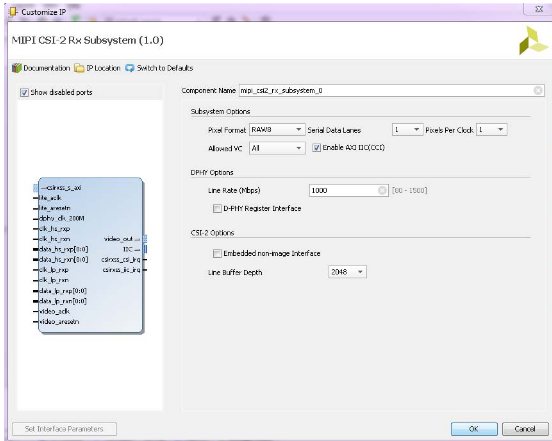
Figure 4-1: Subsystem Customization Screen
