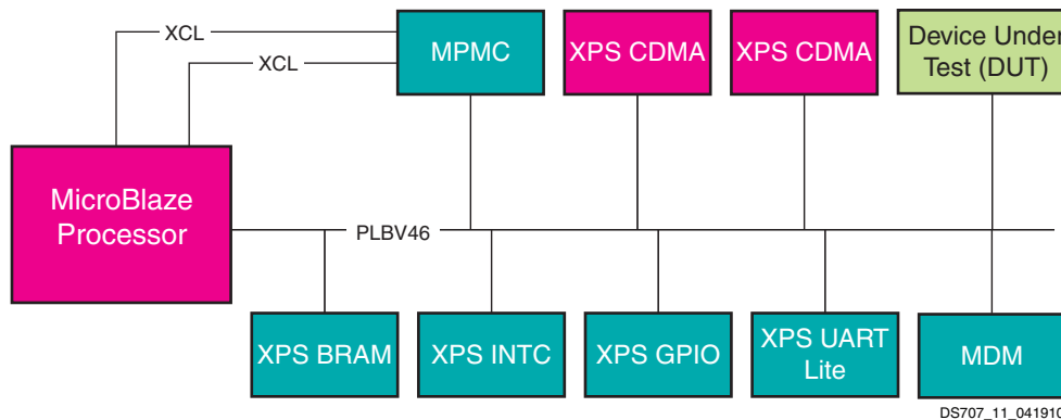
Figure 11: Virtex-5 LX FPGA System with the XPS PS2 Controller as the DUT
