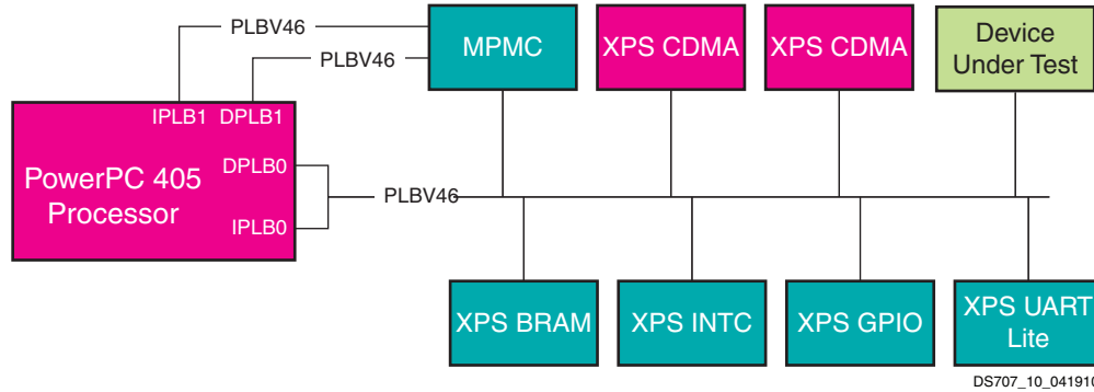
Figure 10: Virtex-4 FX FPGA System with the XPS PS2 Controller as the DUT
