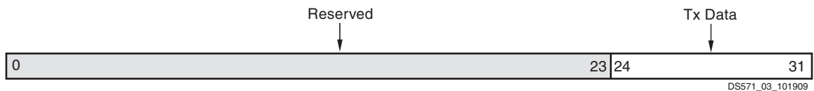
Figure 3: Transmit Data FIFO (C_DATA_BITS = 8)
