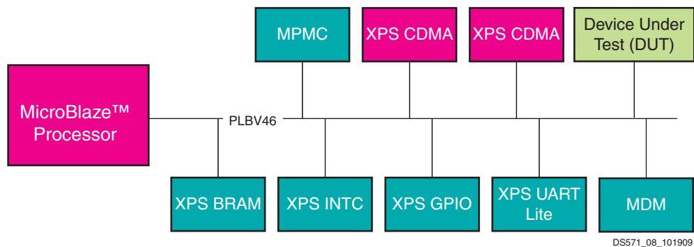
Figure 8: Spartan-3A System with the XPS UART Lite Device as the DUT
