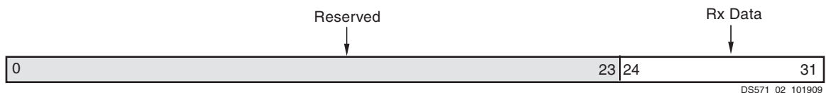
Figure 2: Receive Data FIFO (C_DATA_BITS = 8)
