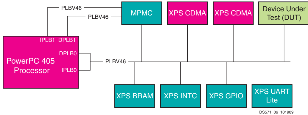
Figure 6: Virtex-4 FX System with the XPS UART Lite Device as the DUT
