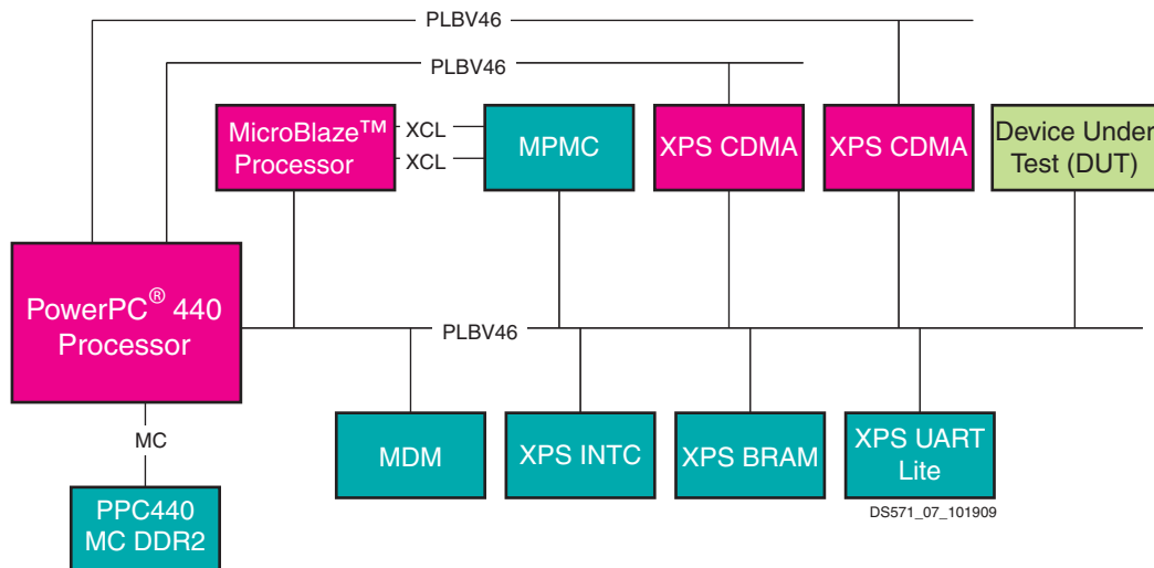
Figure 7: Virtex-5 FX System with the XPS UART Lite Device as the DUT
