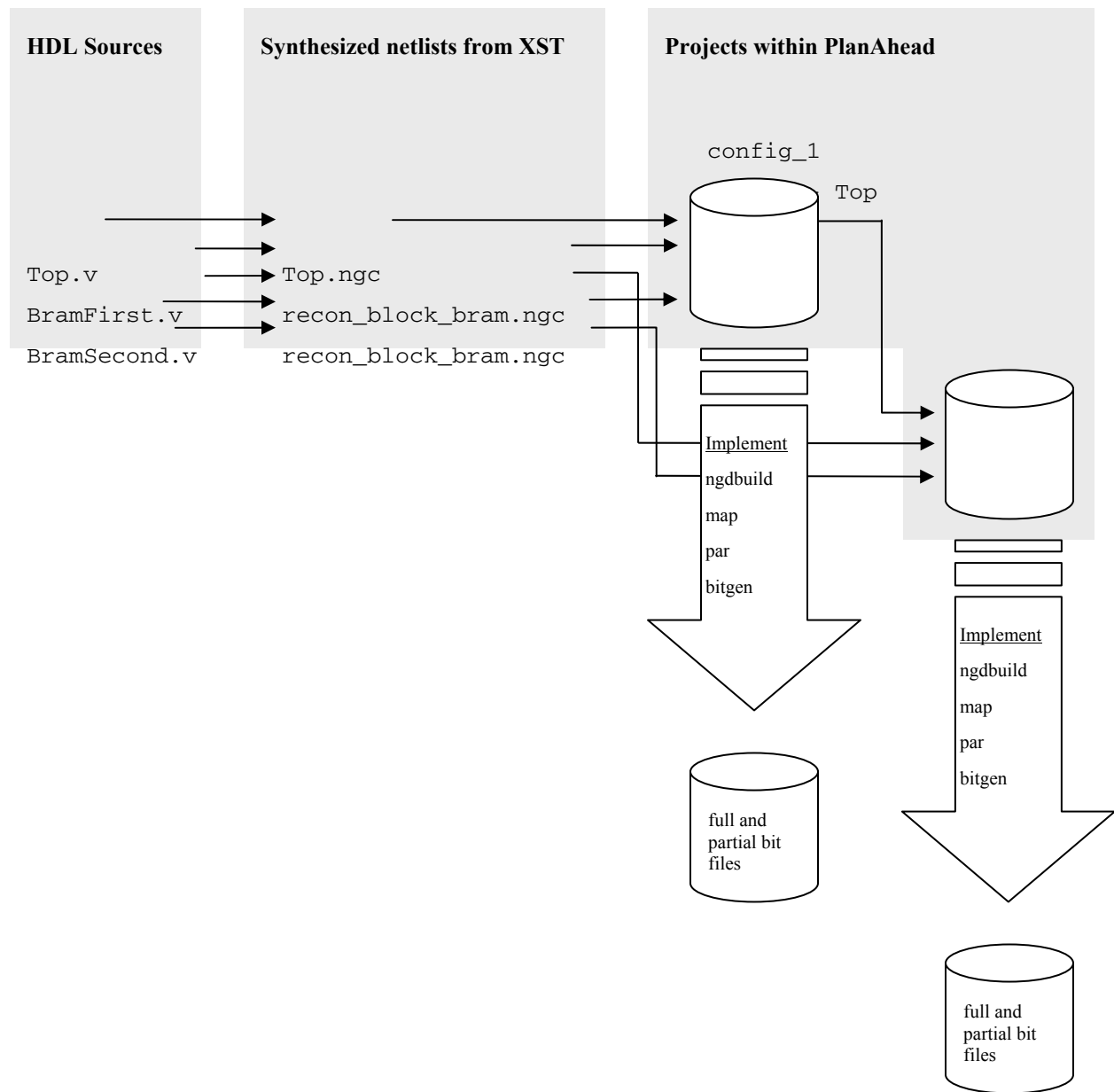
Figure 2: Software Flow Overview
