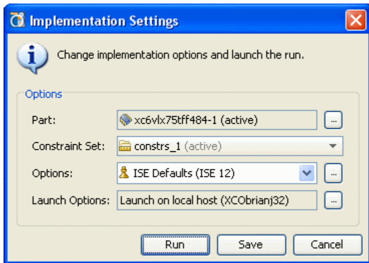
Figure 18: Implementation Settings Dialog Box
