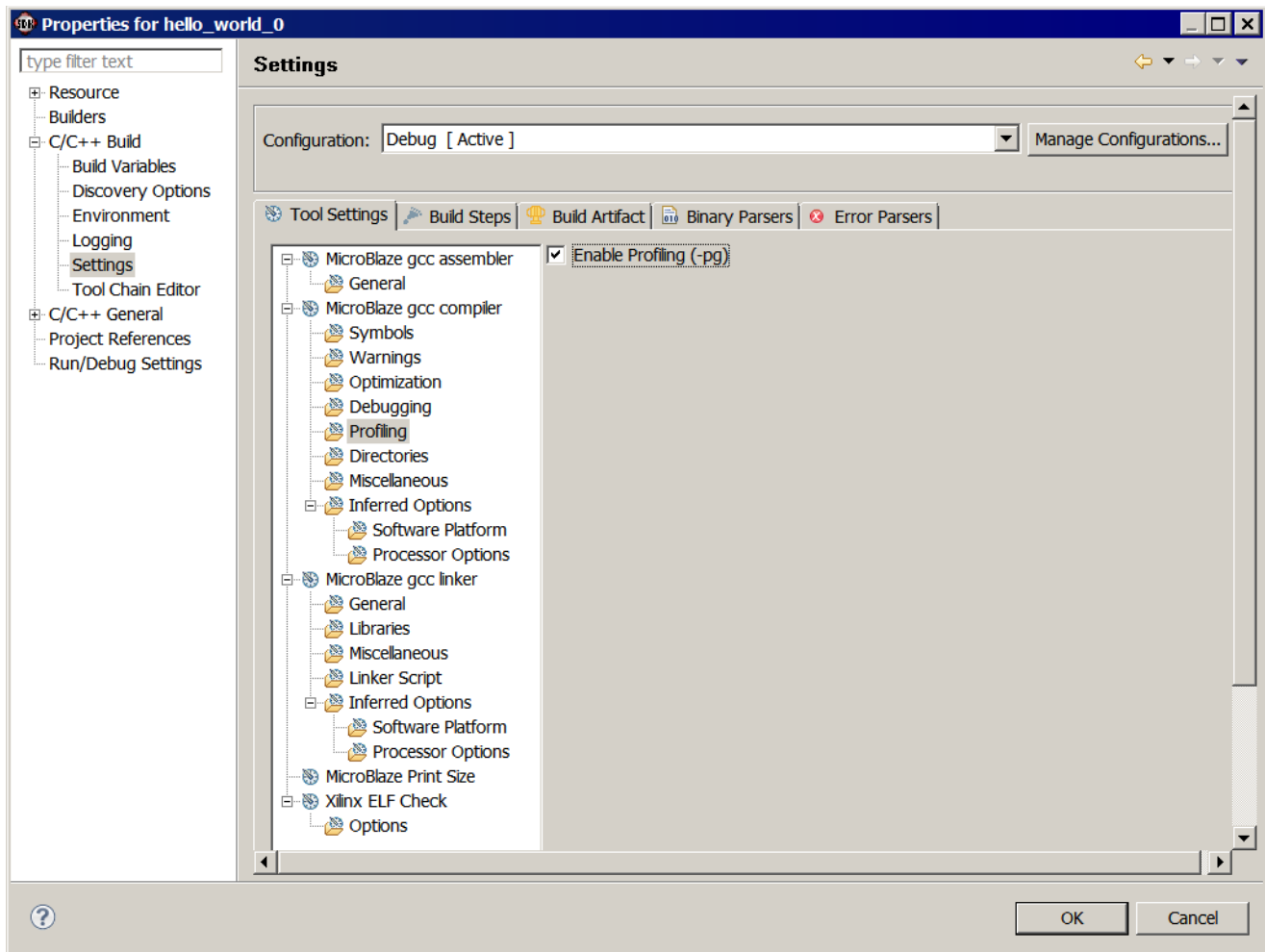
Figure 2-3: Properties Dialog Box with Profiling Enabled
