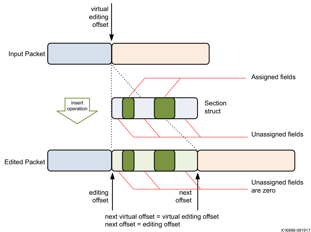
Figure 3-5: insert Method
