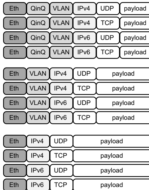
Figure 3-10: Packet Formats for the Five-level Protocol Stack
