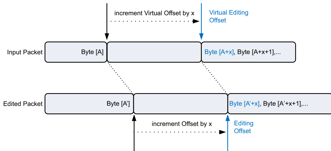
Figure 3-1: increment_offset Method
