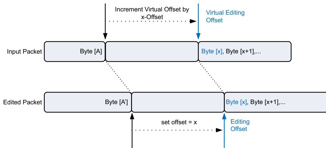
Figure 3-2: set_offset Method
