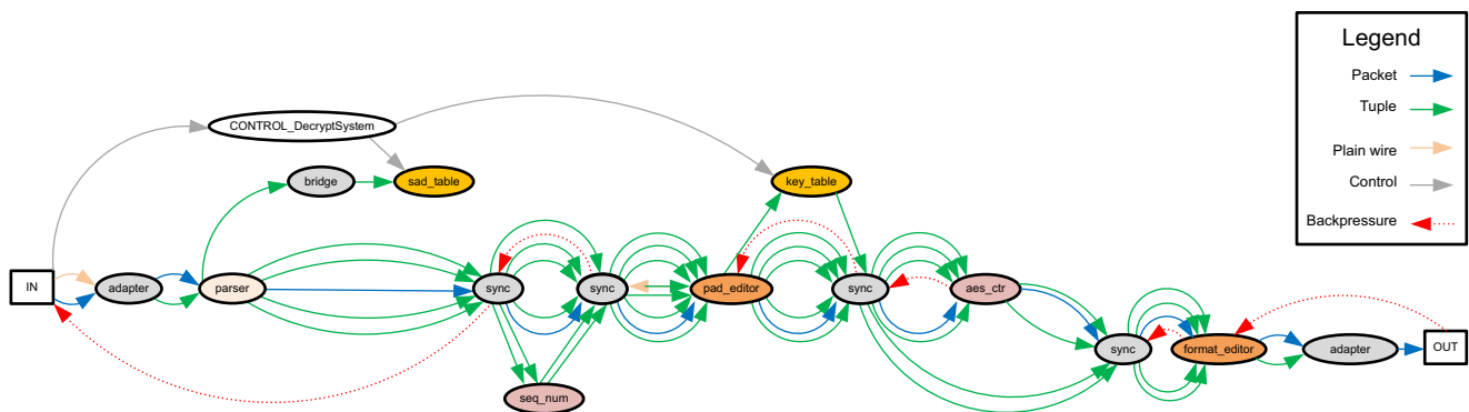
Figure 4-5: More Complex Elaborated/RTL Dataflow Graph Example
