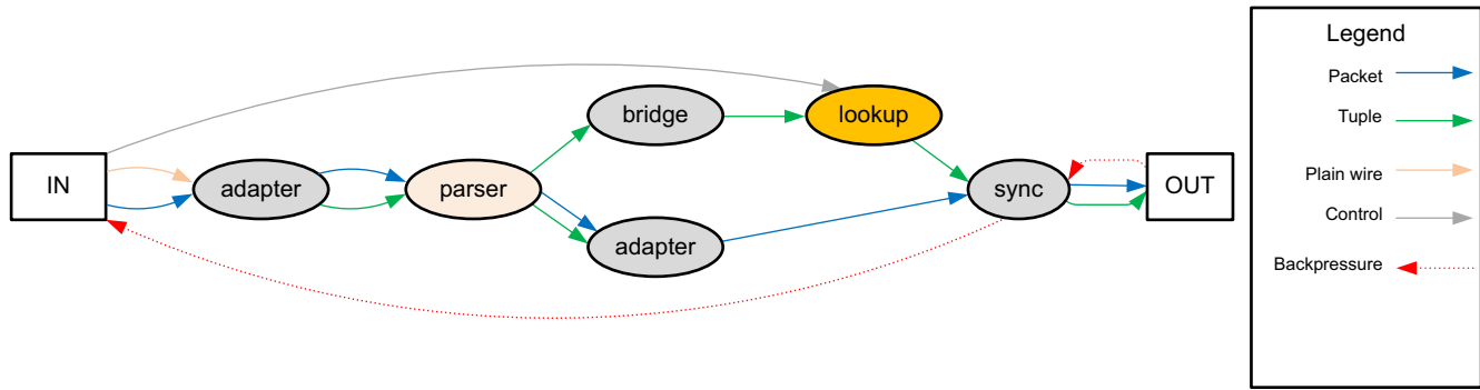
Figure 4-4: Simple Elaborated/RTL Dataflow Graph Example
