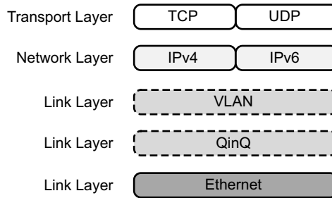
Figure 3-9: Five-level Protocol Stack
