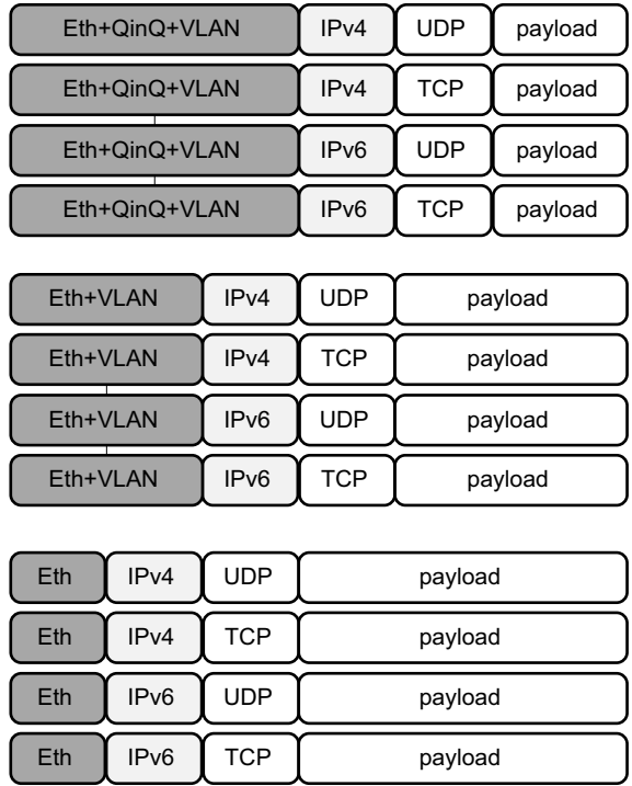
Figure 3-14: Simplified Packet Format
