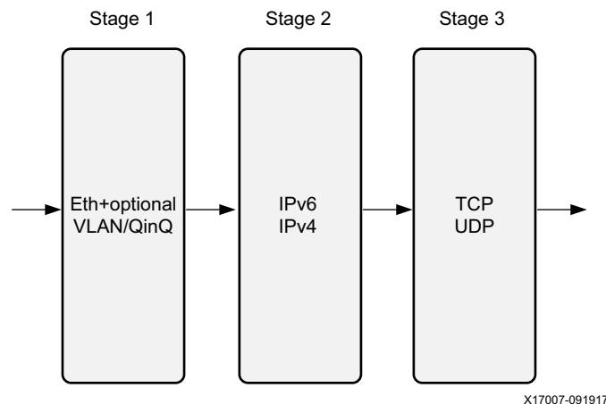
Figure 3-13: Optimized Parser
